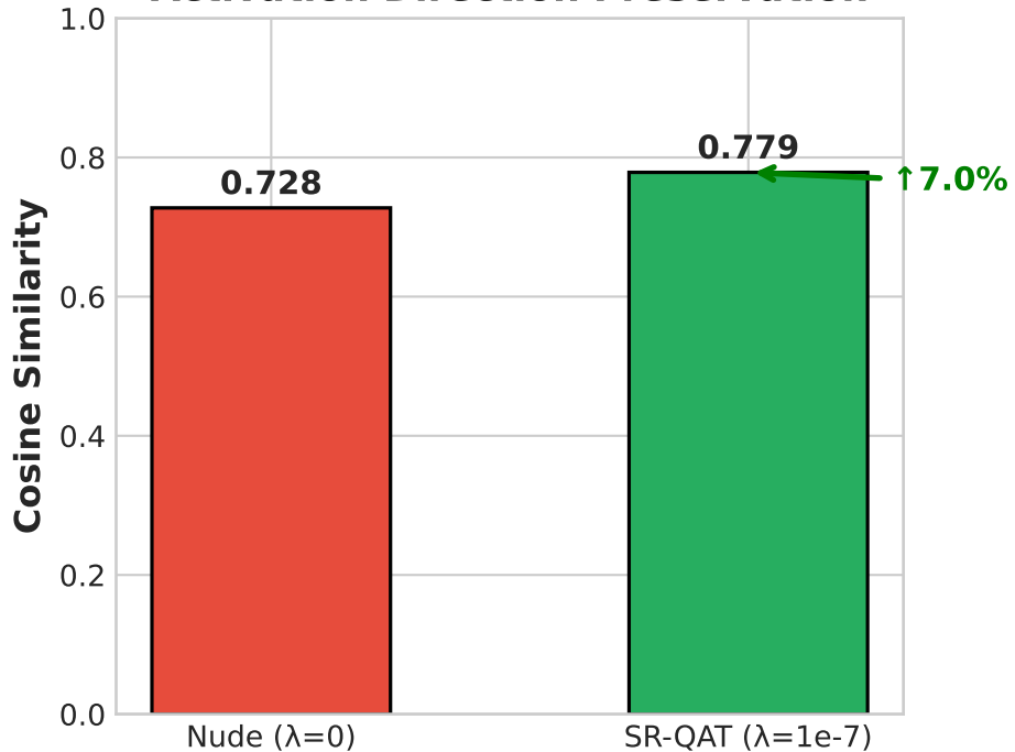
Activation Direction Preservation
