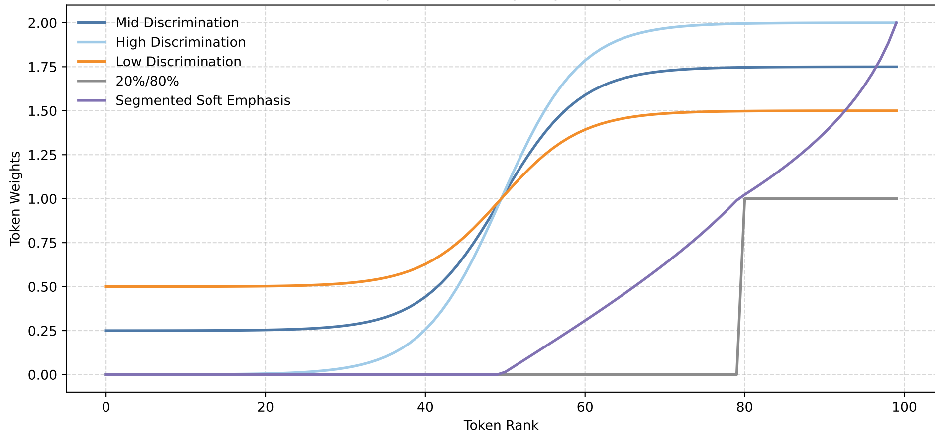
Adaptive Token Weighting Strategies
