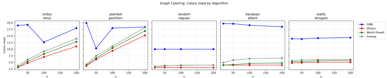
Figure 3: Colors used by each algorithm across graph families. DSatur consistently uses the fewest colors; the GNN uses 3\text{--}4\times more.
