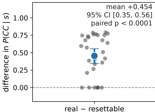
(b) Per-seed difference
