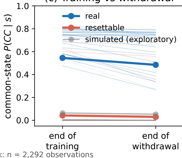
(c) Training vs withdrawal
