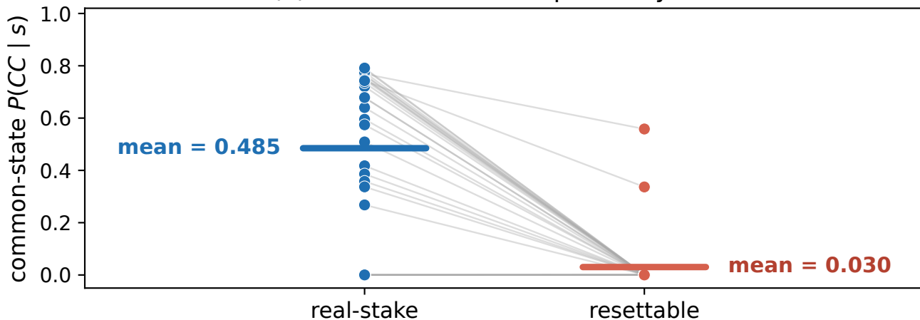
(a) End-of-withdrawal, paired by seed
