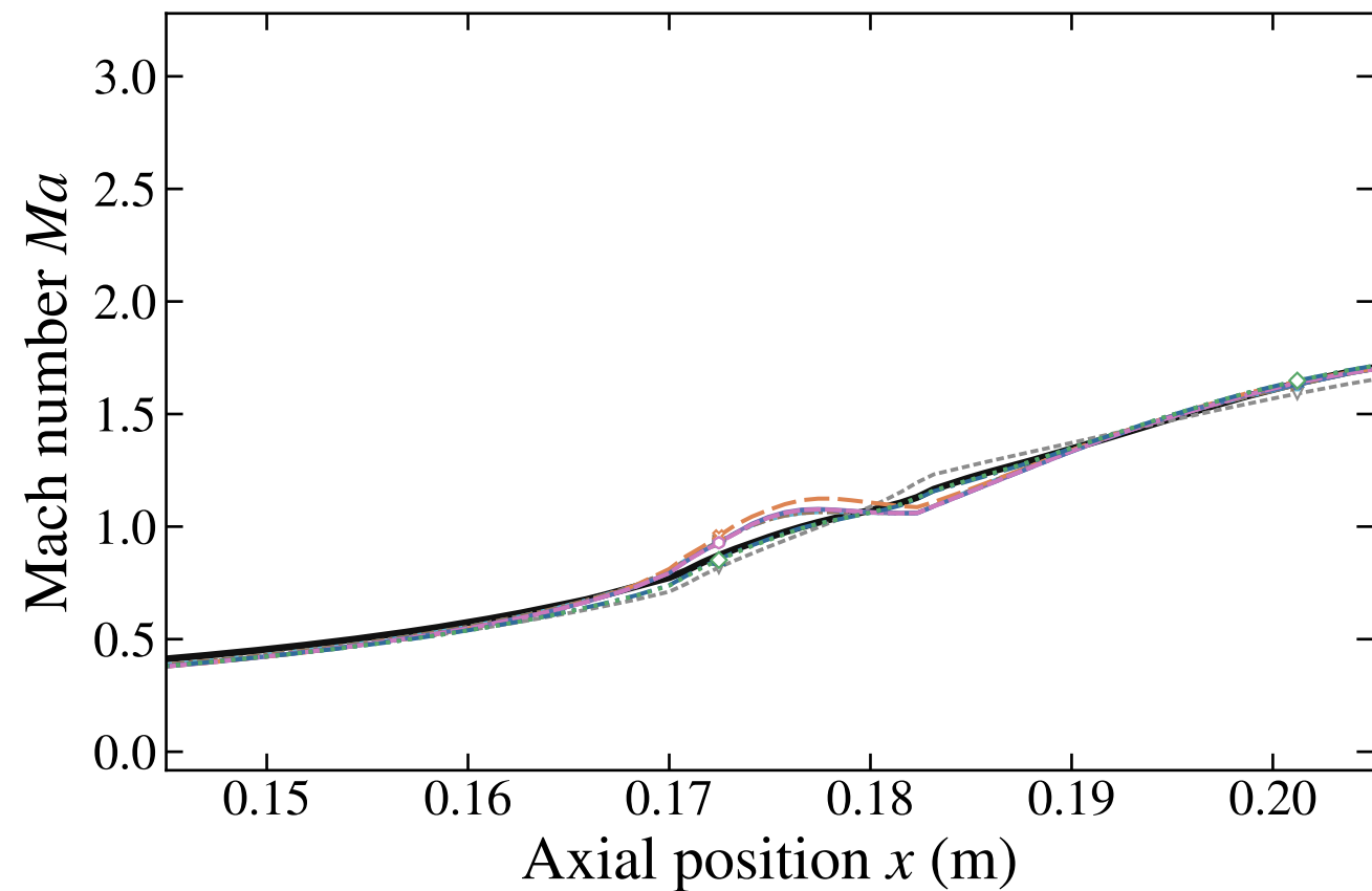
Throat Mach number
