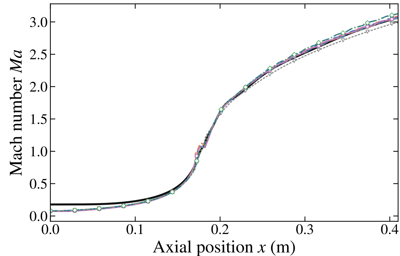
Full axial Mach number
