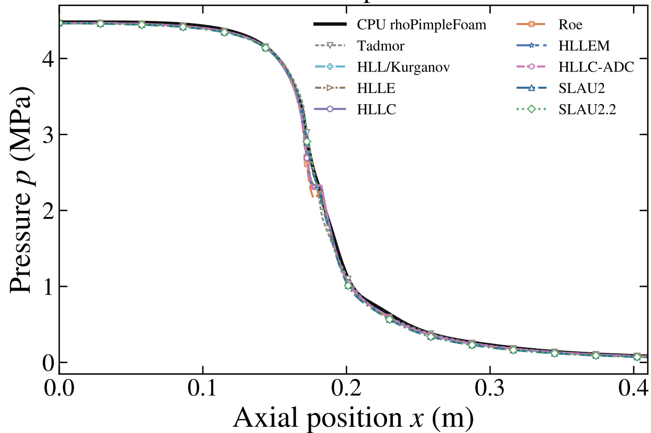
Full axial pressure
