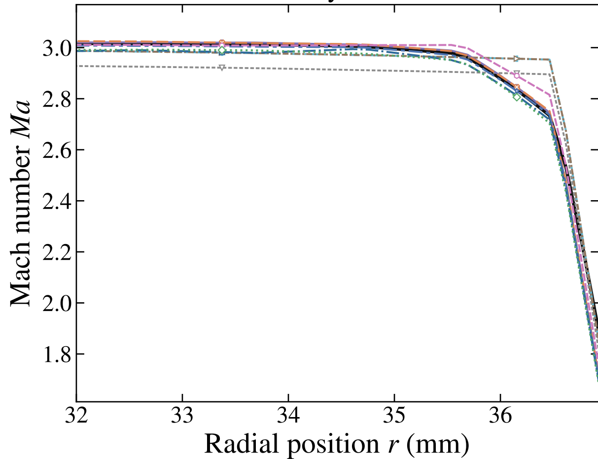
Wall-layer detail
