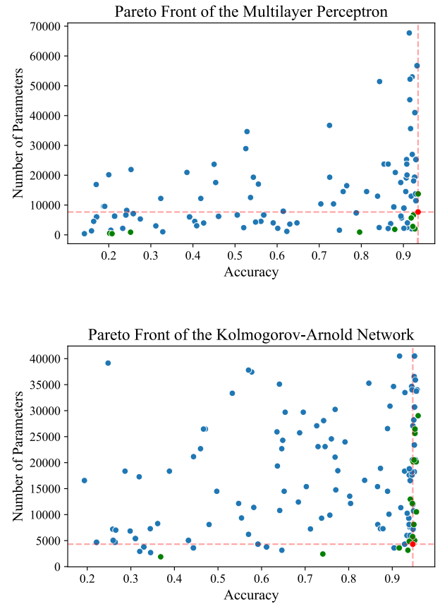
FIGURE 5. 2D representation of a 3D Pareto front that shows the mean accuracy between upper body and lower body predictions against number of parameters. Green points are inside the front, and red points correspond to the chosen parameters.
