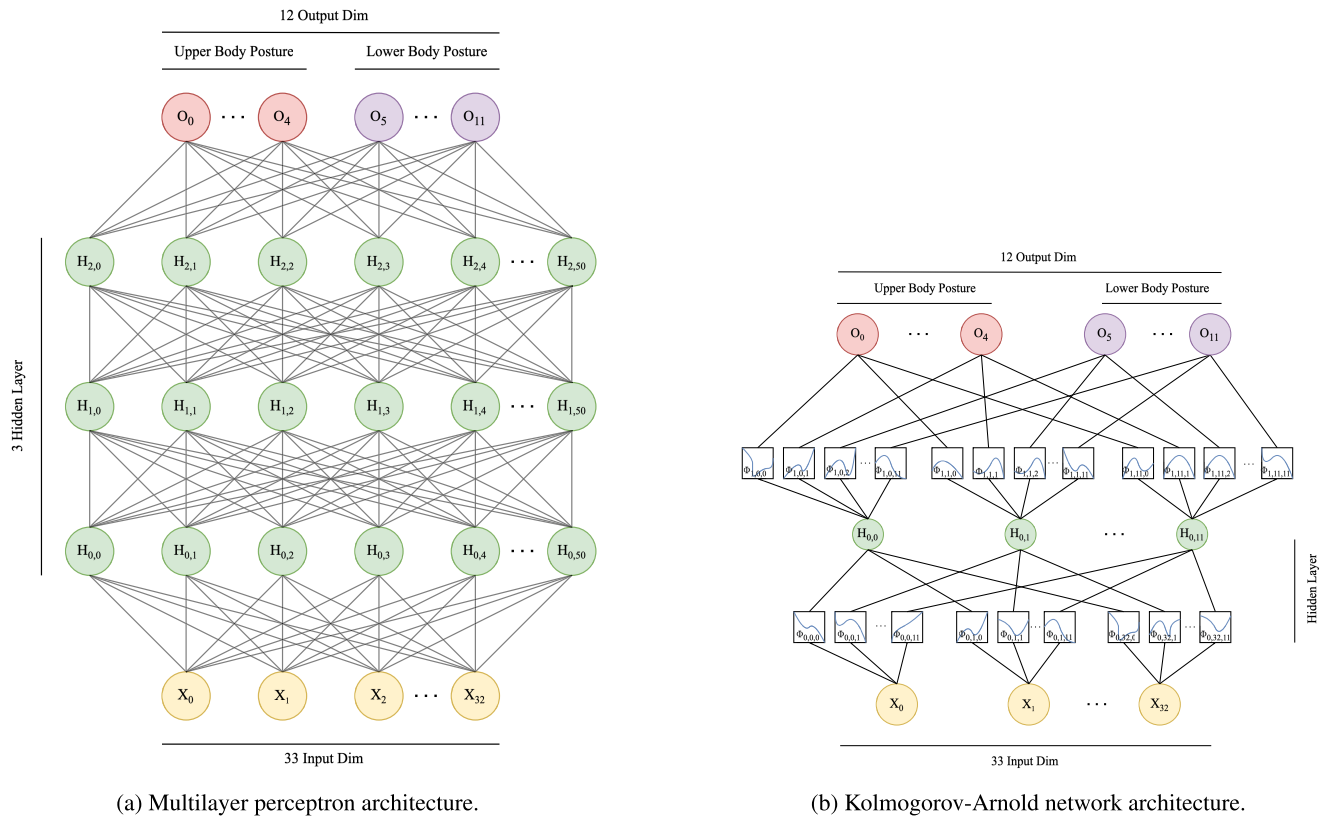
FIGURE 4. Comparison of model architectures: (a) Multilayer perceptron (MLP) with three hidden layers, and (b) Kolmogorov-Arnold network (KAN) with a single hidden layer. Both architectures have 33 input dimensions corresponding to skeletal keypoints and 12 output dimensions representing upper and lower body posture classifications.
