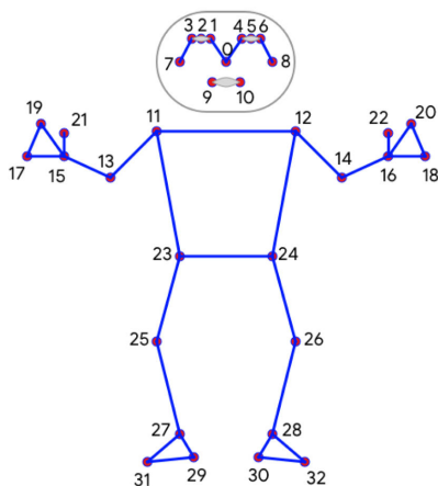
FIGURE 2. Keypoint topology used by BlazePose [28].
