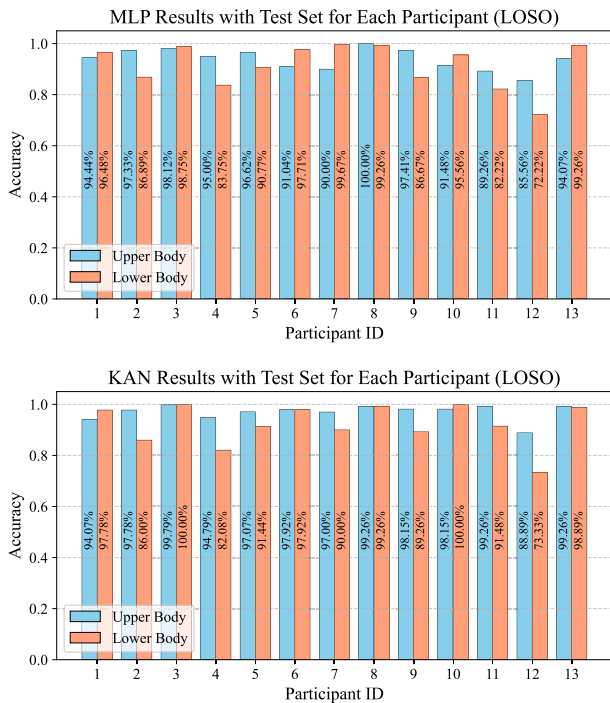
FIGURE 6. Comparison of MLP and KAN model performance using LOSO cross-validation. The graphs show the accuracy of upper body and lower body posture prediction for each of the 13 participants.
