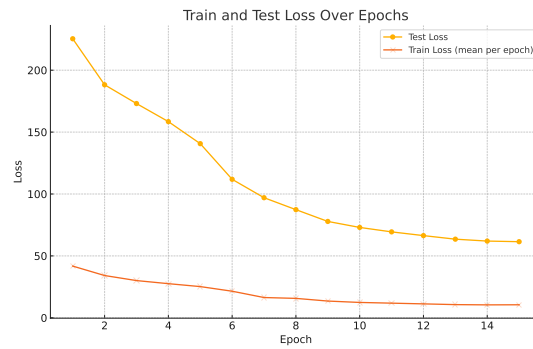
Figure 2: The training process of the VAE layer. The reconstruction error of the hidden state vector calculates the loss. The training process is stable and converges quickly.
