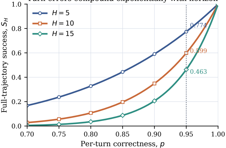
Turn errors compound exponentially with horizon
