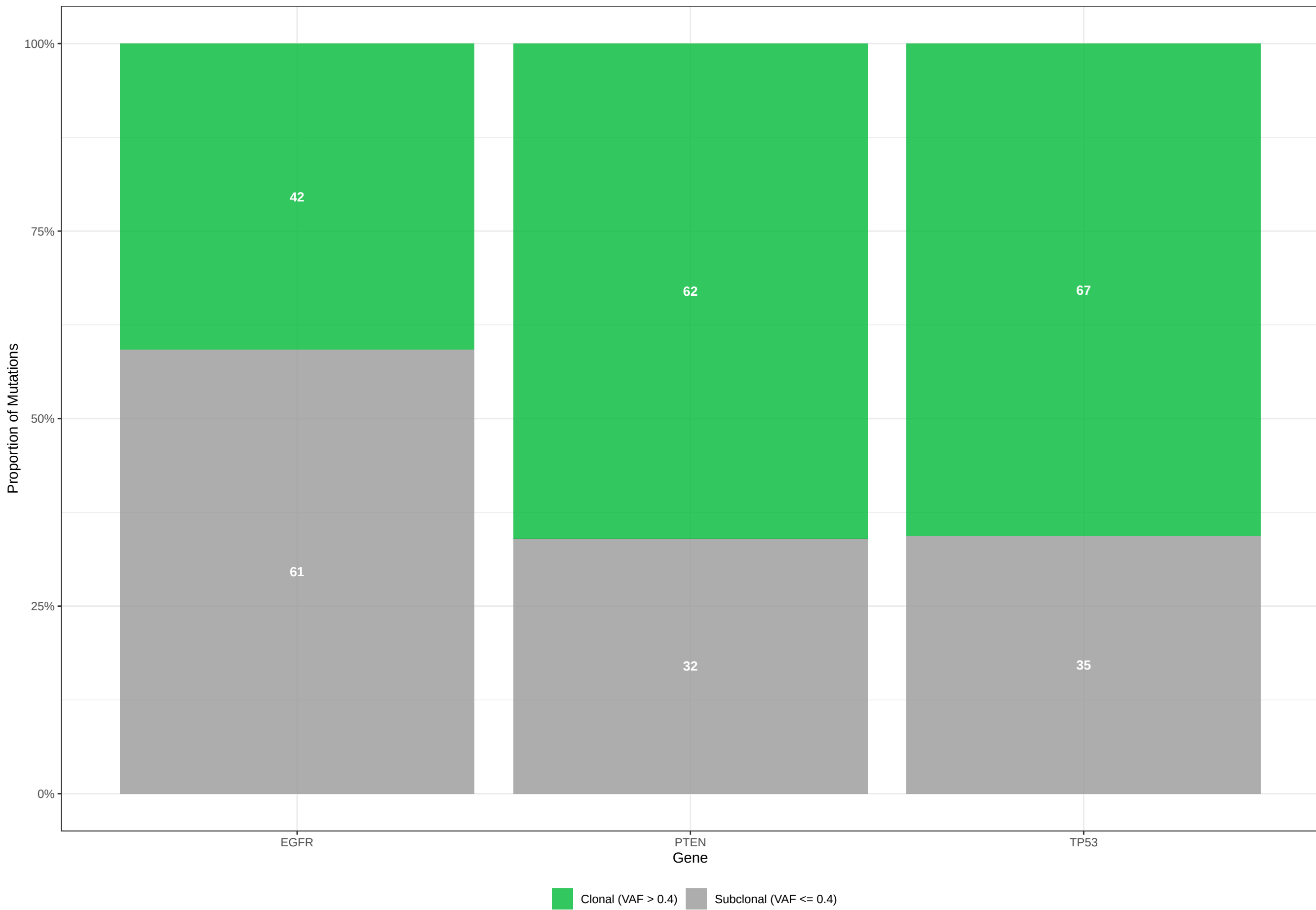
Clonality Proportions by Gene
