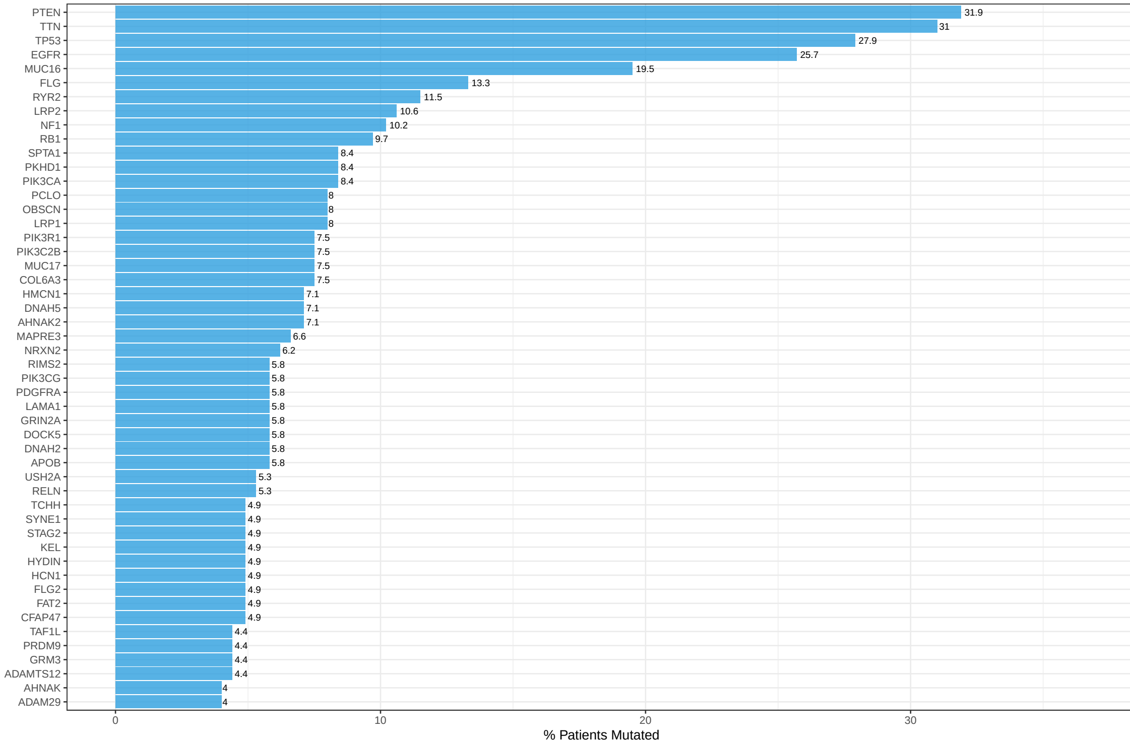
Supplementary Figure 1: Top 50 Mutated Genes
