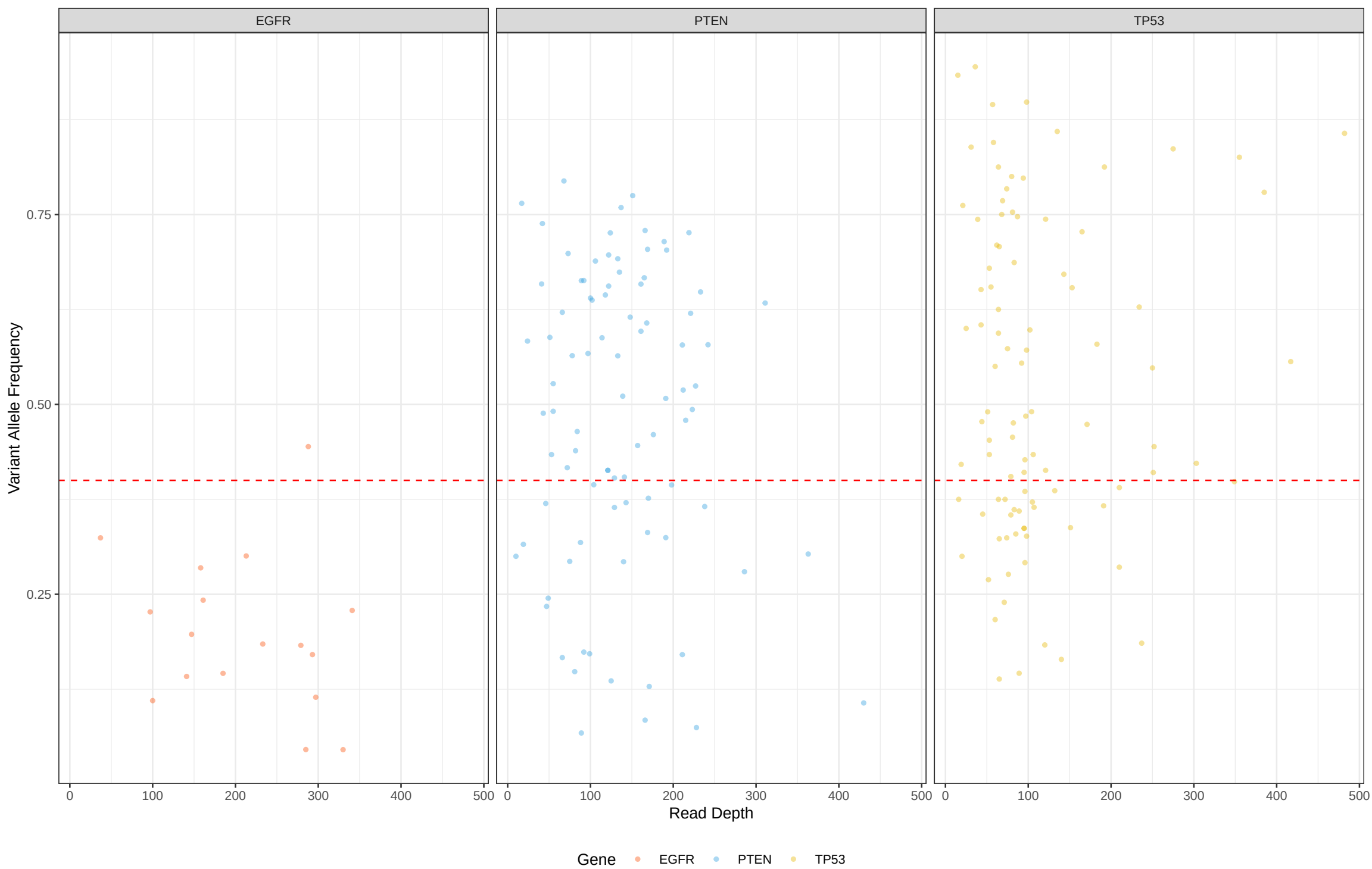
Supplementary Figure 2: VAF vs Read Depth
