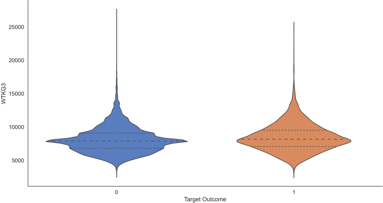
Comparative Density: WTKG3
