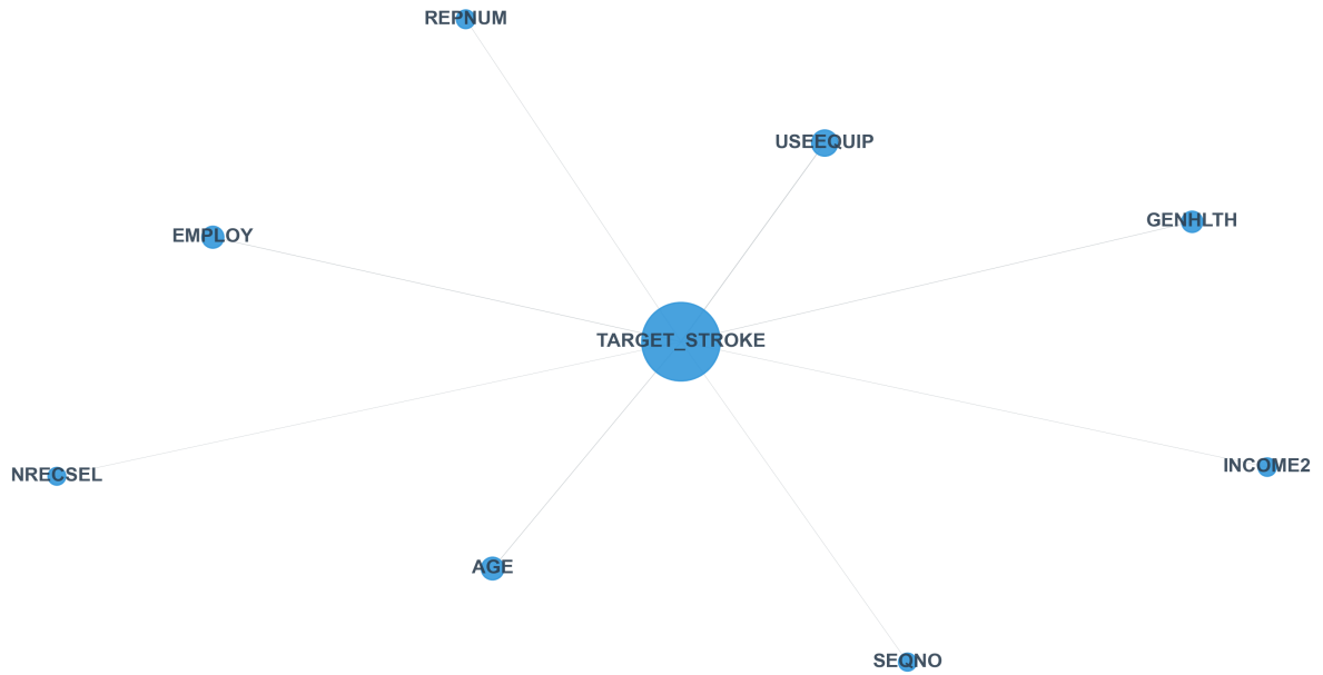
Predictor Influence Network: 2008.csv
