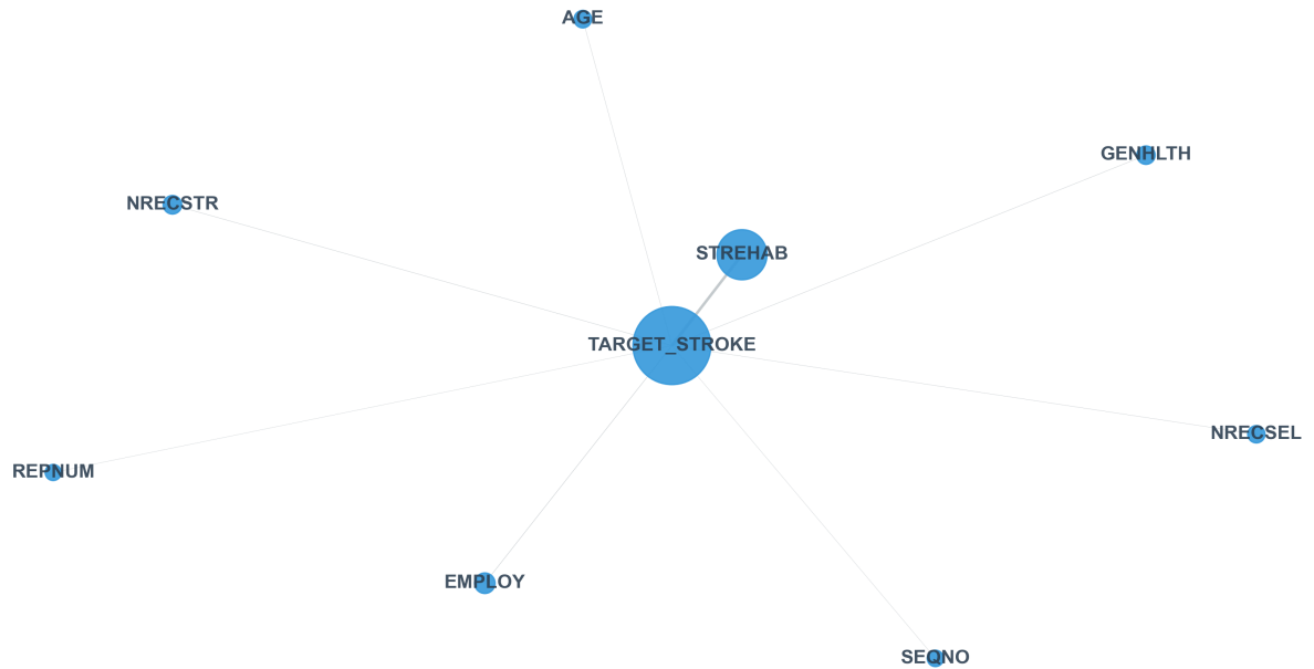
Predictor Influence Network: 2005.csv
