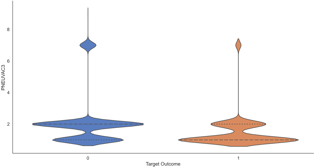
Comparative Density: PNEUVAC3
