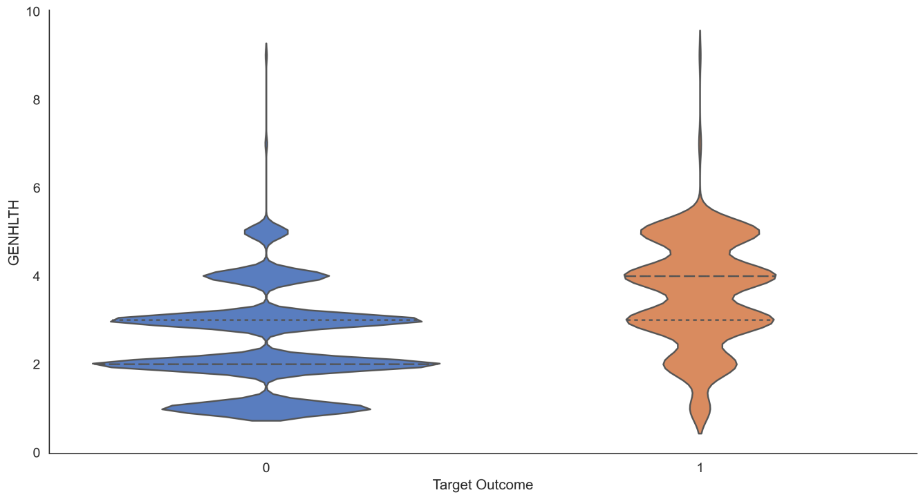
Comparative Density: GENHLTH
