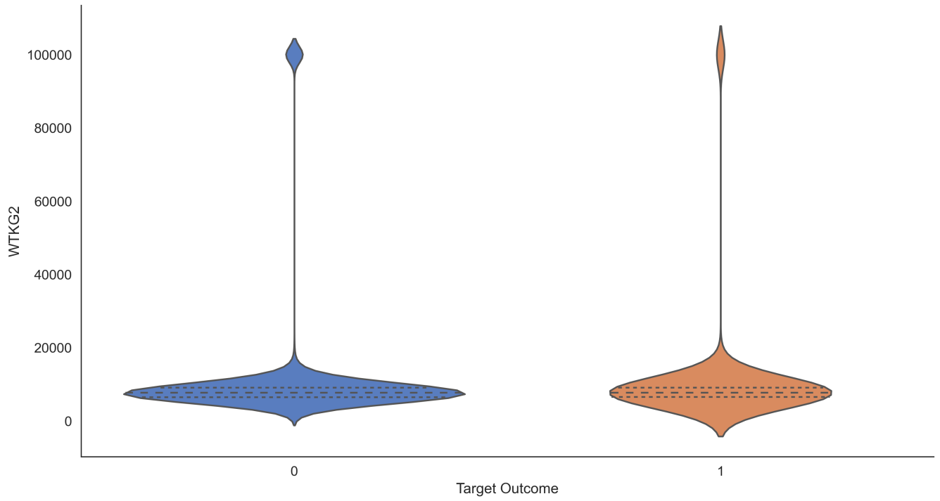
Comparative Density: WTKG2
