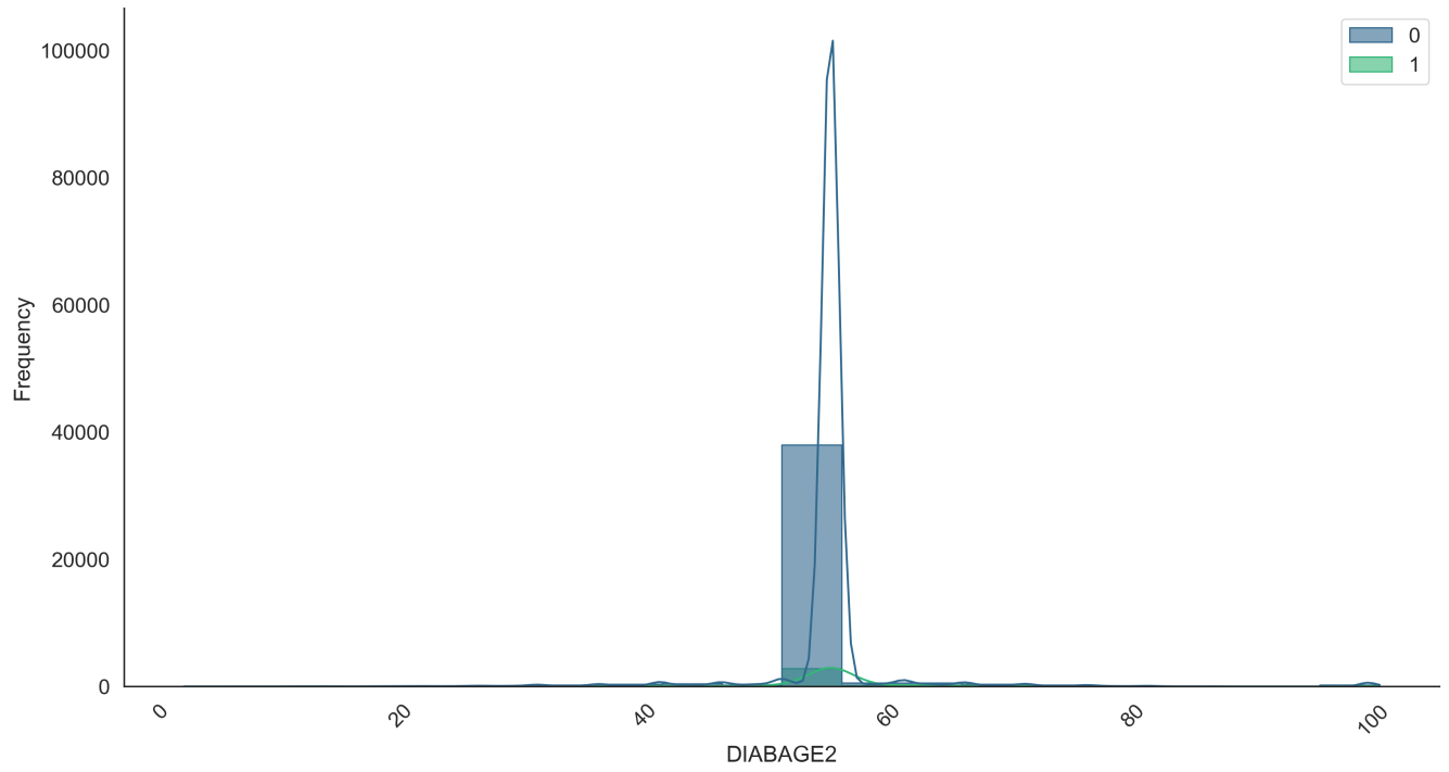
Distribution Analysis: DIABAGE2
