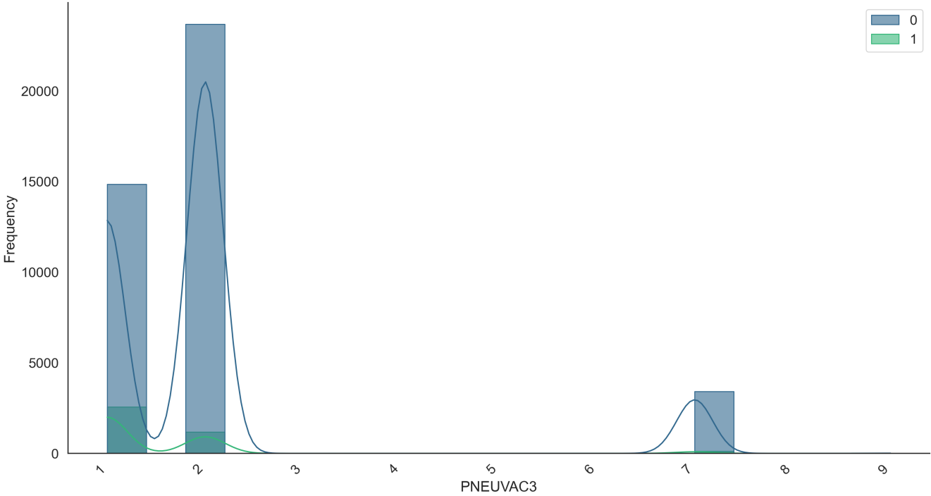
Distribution Analysis: PNEUVAC3
