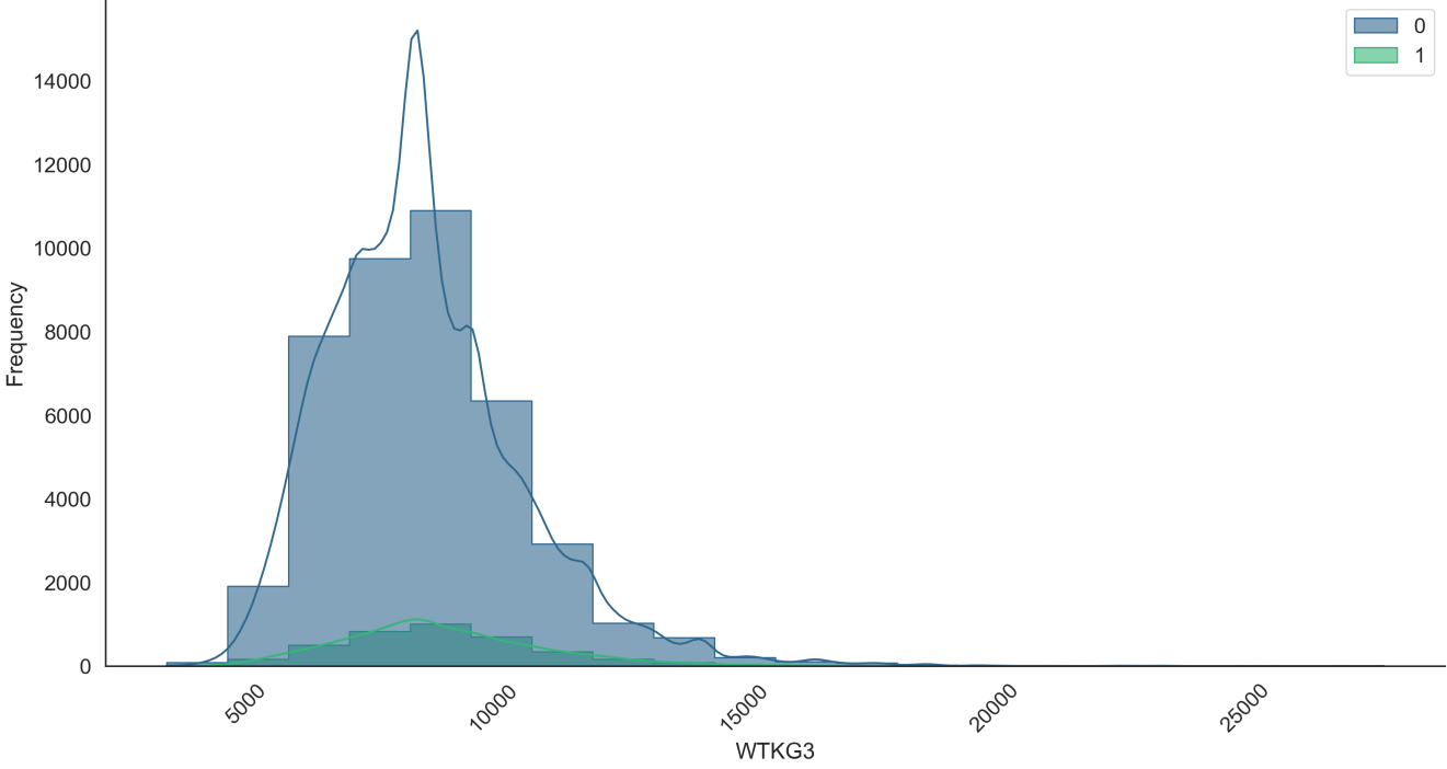
Distribution Analysis: WTKG3
