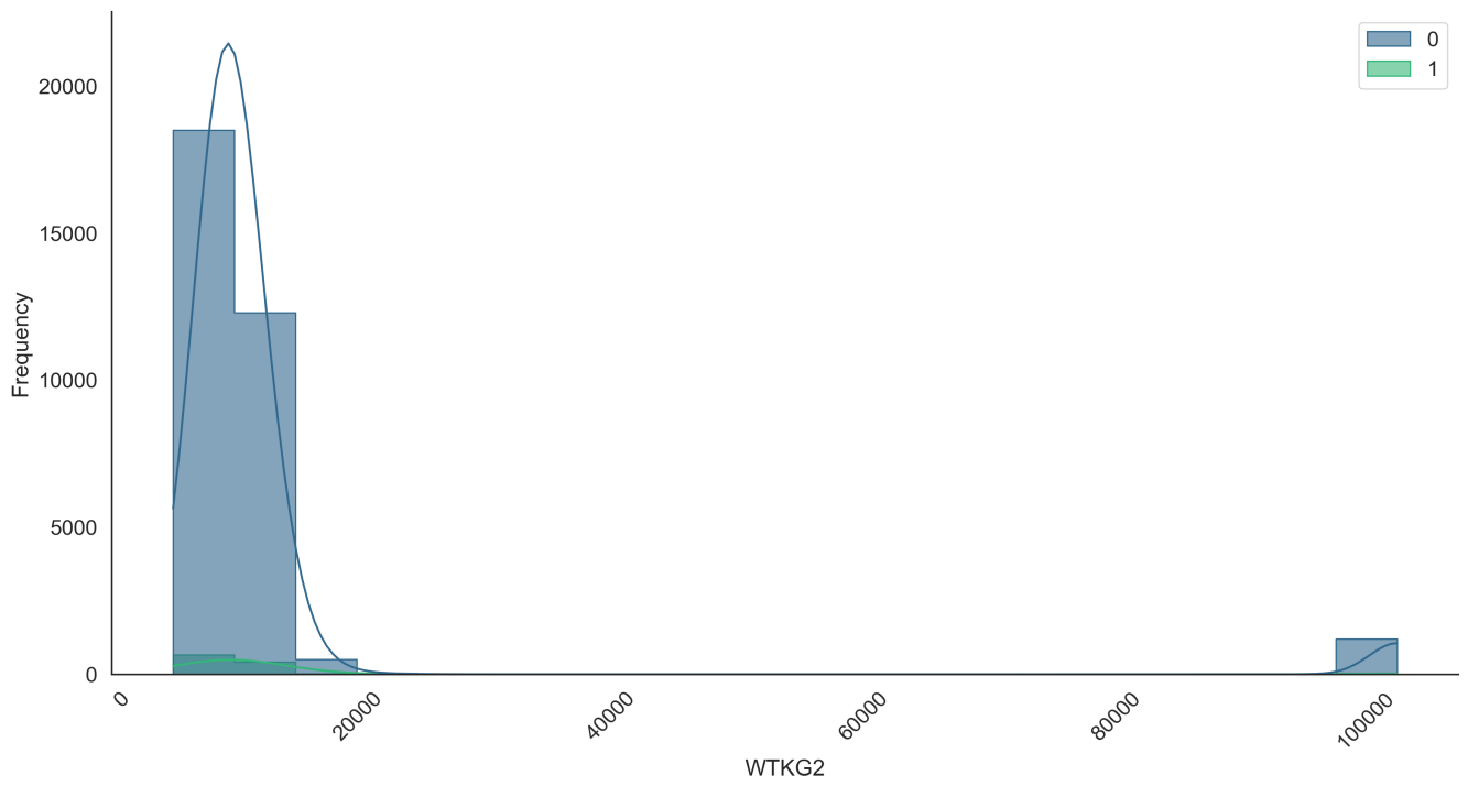
Distribution Analysis: WTKG2
