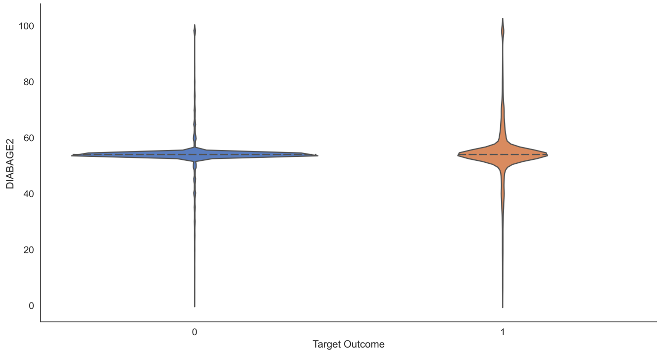
Comparative Density: DIABAGE2
