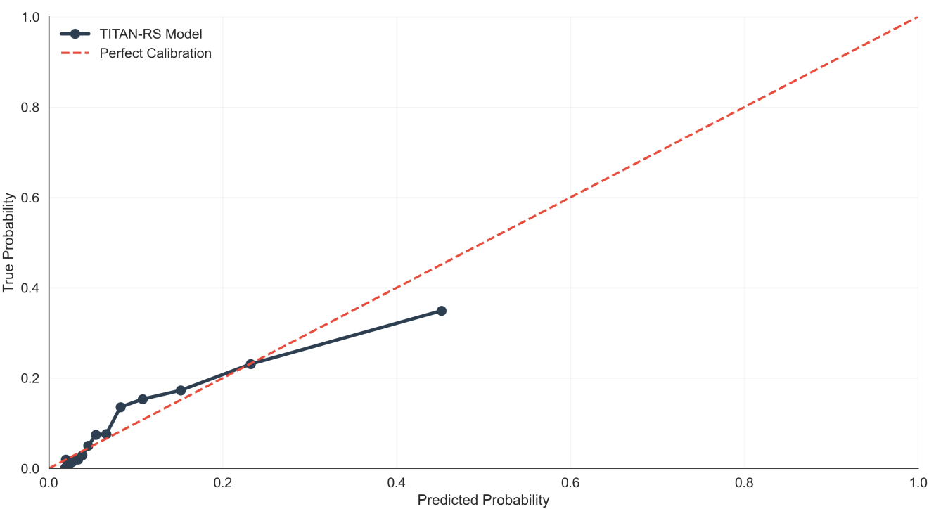
Reliability Diagram (Calibration)
