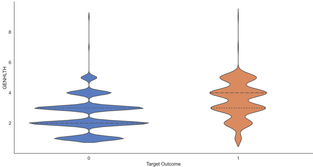
Comparative Density: GENHLTH
