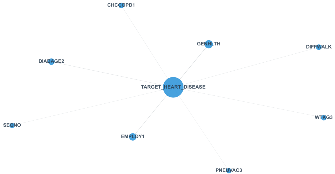
Predictor Influence Network: 2016.csv
