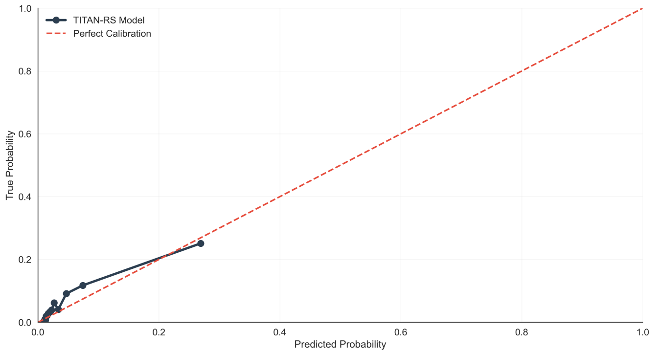
Reliability Diagram (Calibration)
