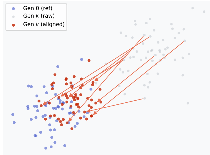
3. Temporal alignment ( \lambda = 0.8 , Eq. 1)
