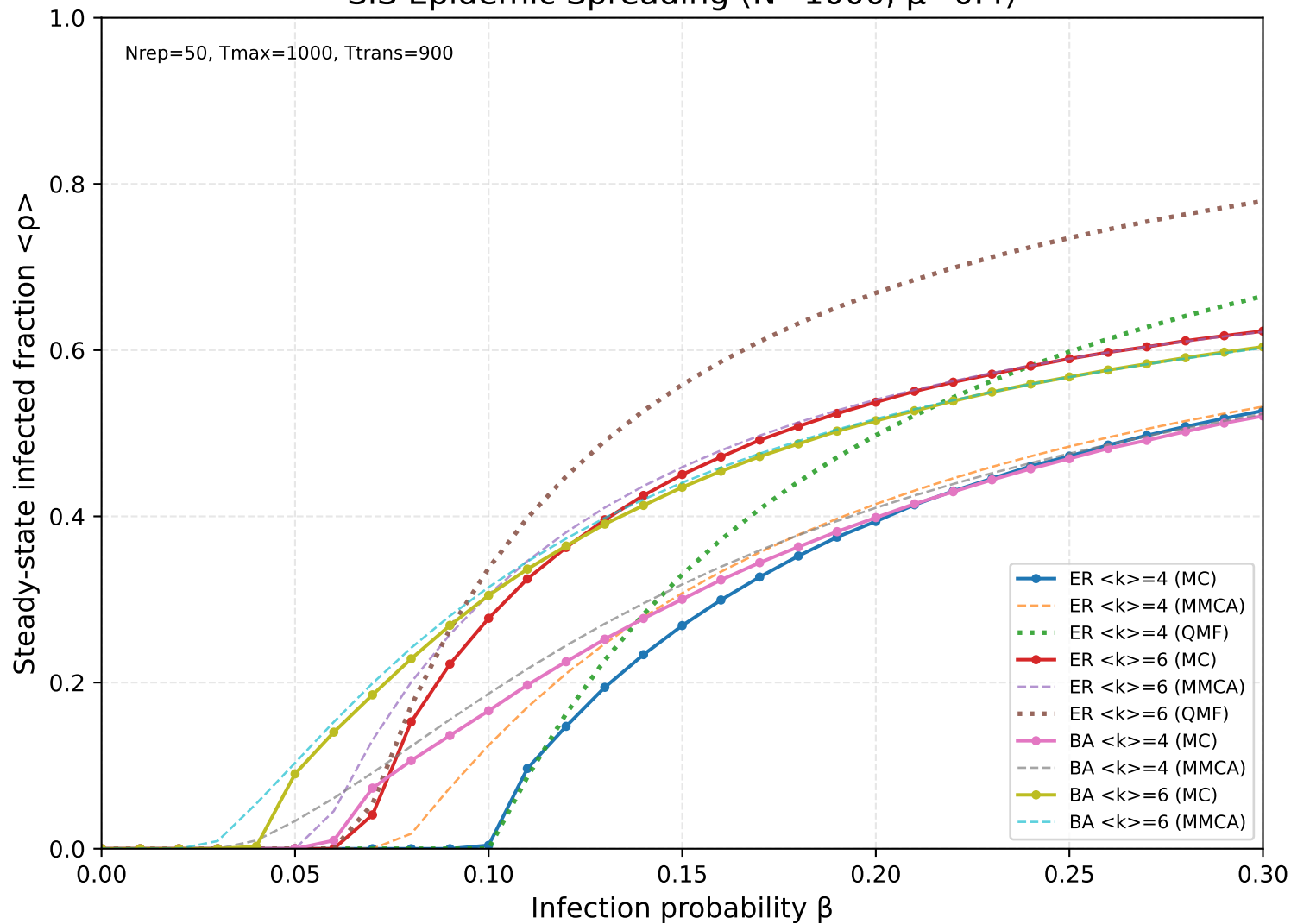
SIS Epidemic Spreading (N=1000, \mu=0.4 )
