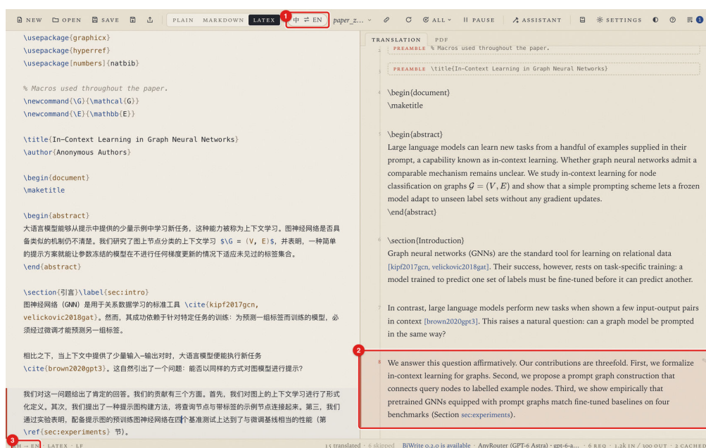
Figure 14 A Chinese file: (1) the button reads 中 \Rightarrow EN and is not swapped, (2) the English translation on the right, (3) zh en in the status bar
