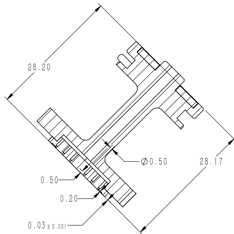
SECTION AC-AC
