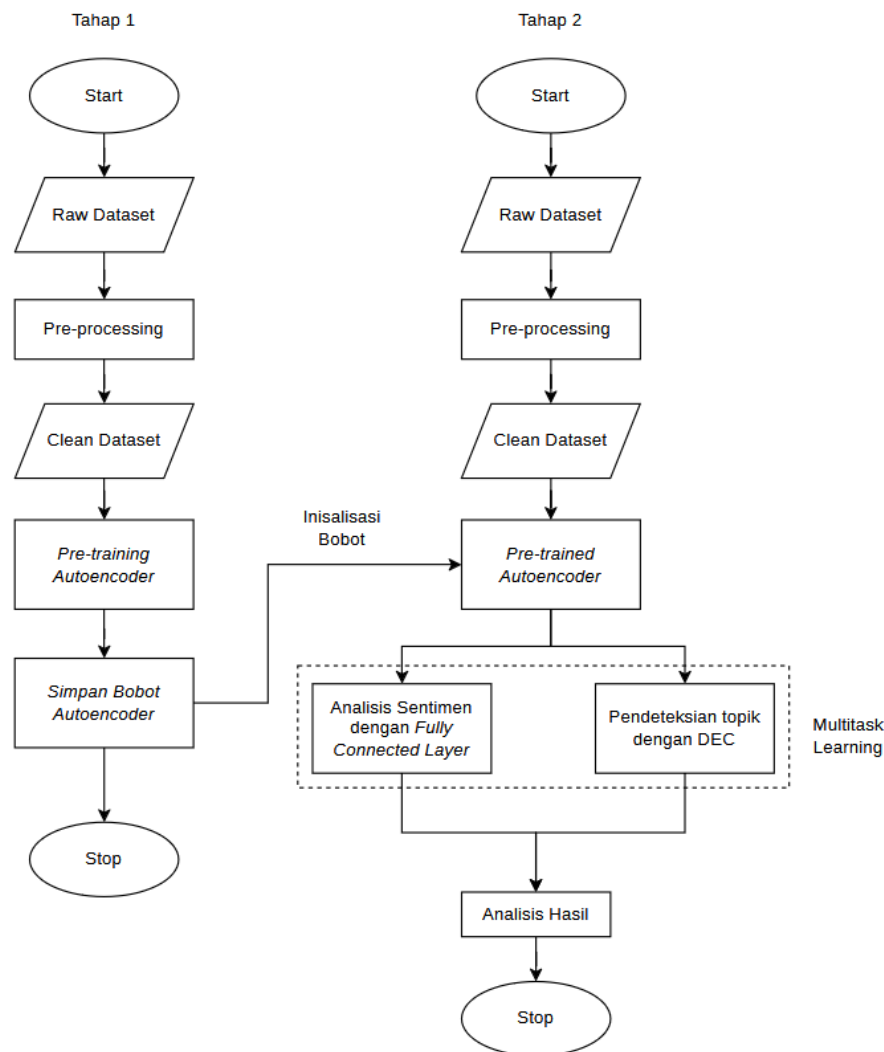
Gambar 4.1: Diagram alur simulasi penelitian.
