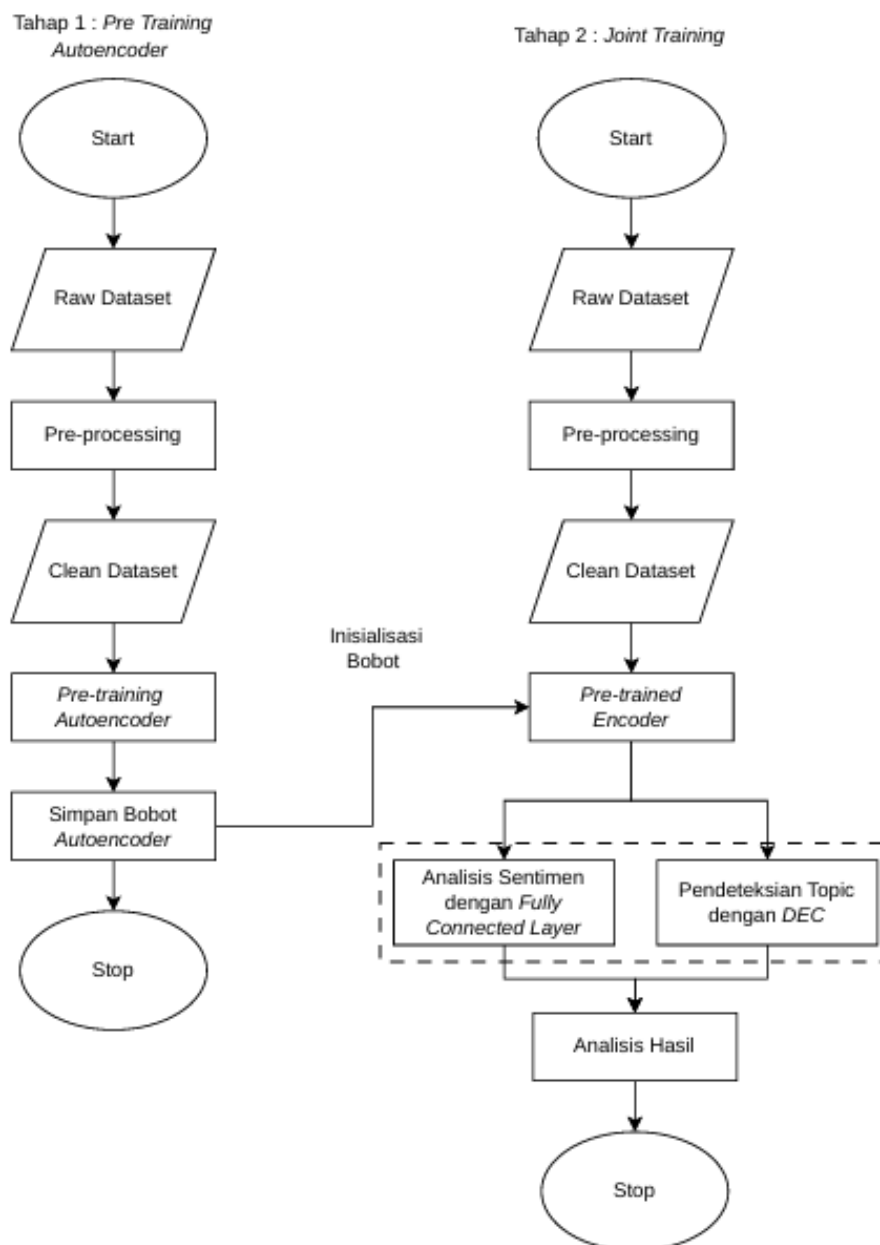
Gambar 4.1: Diagram alur simulasi penelitian.
