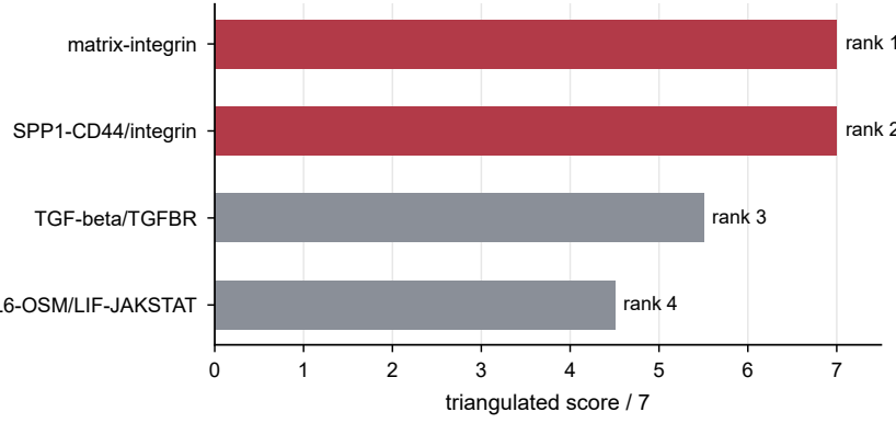
Perturbation-priority rank
