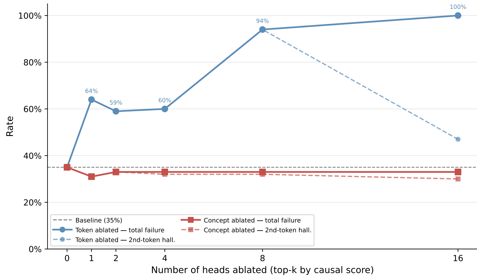
Llama-3.1-8B: Effect of head ablation (solid = total failure, dashed = 2nd-token hallucination)
