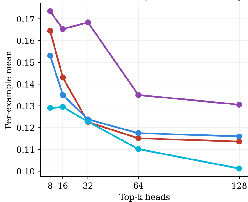
Olmo-3-1025-7B - Concept LTM (value-weighted)
