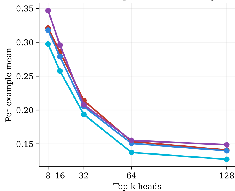
Qwen3-8B - Concept LTM (value-weighted)
