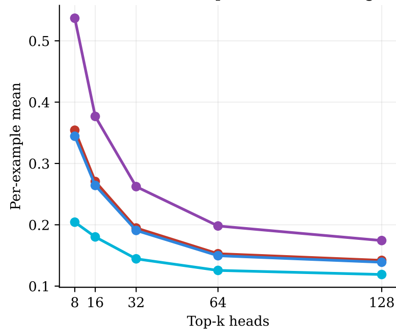
Llama-3.1-8B - Concept LTM (value-weighted)
