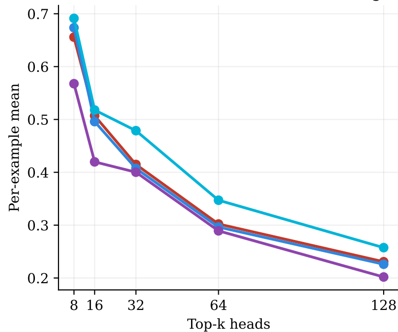
Olmo-3-1025-7B - Token NTM (value-weighted)
