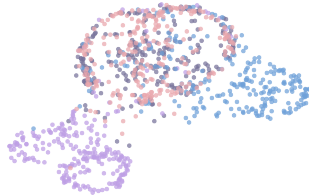
PatchAE reconstruction
