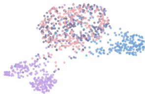
Observed cells
