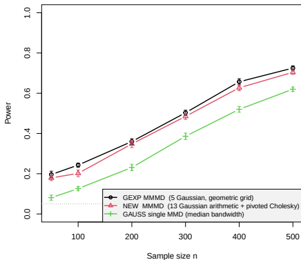
Figure 1(b) reproduction (Gaussian Scale, d = 2 ) with new method
