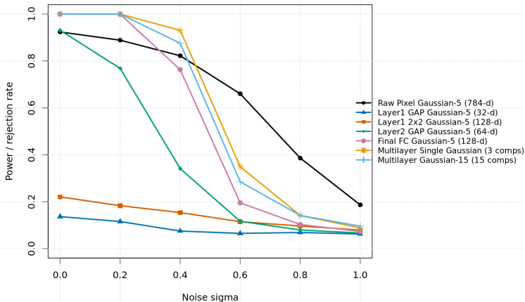
MNIST CNN Embedding MMD Power Comparison
