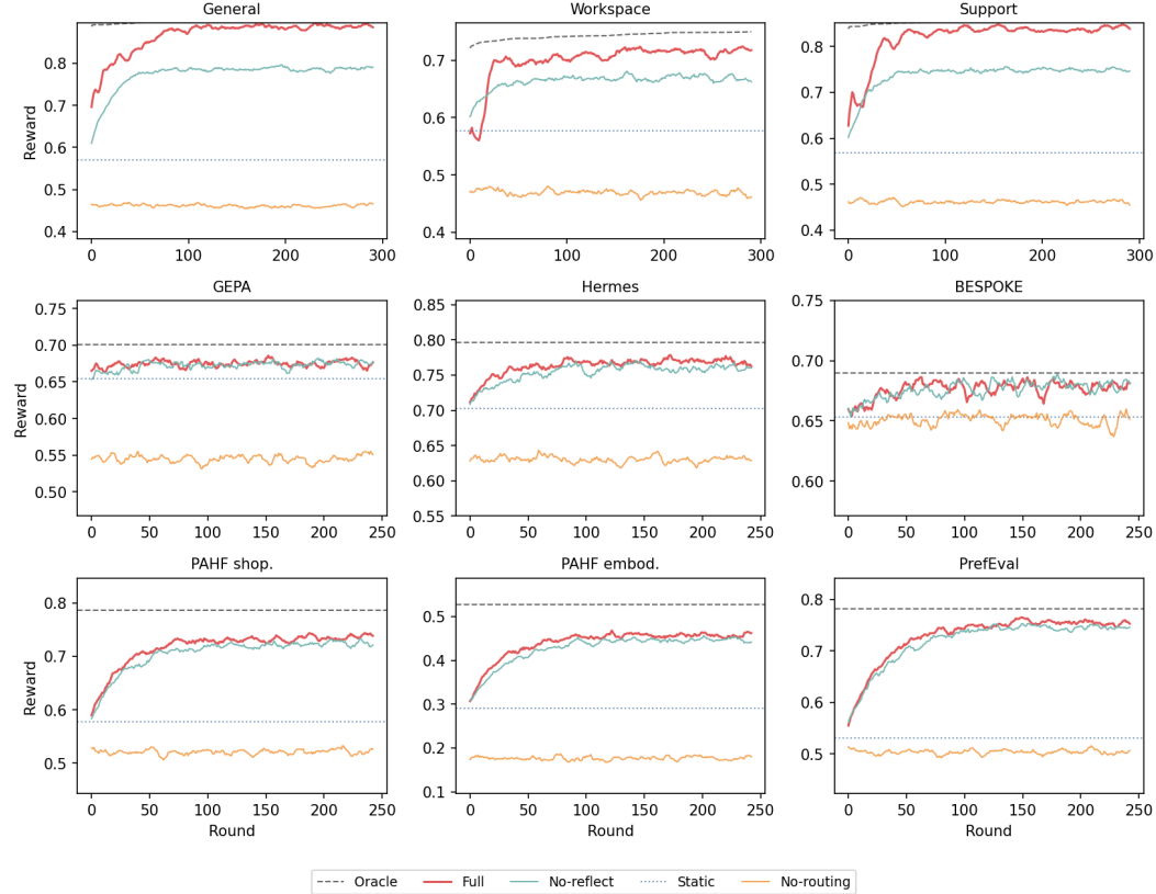
Figure 2: Per-round reward for all nine benchmarks ( 3 \times 3 grid). Five variants shown: Full (red; concat features, gated reflection, LinUCB), No-reflect (teal; frozen archive, \vec{G}_T=0 ), No-routing (orange; uniform-random selection, \Delta_{\text{route}} \rightarrow 0 ), Static (gray dotted; best single candidate for all users), Oracle (black dashed; per-user optimum). Top row: synthetic; middle and bottom: framework and real-data benchmarks.
