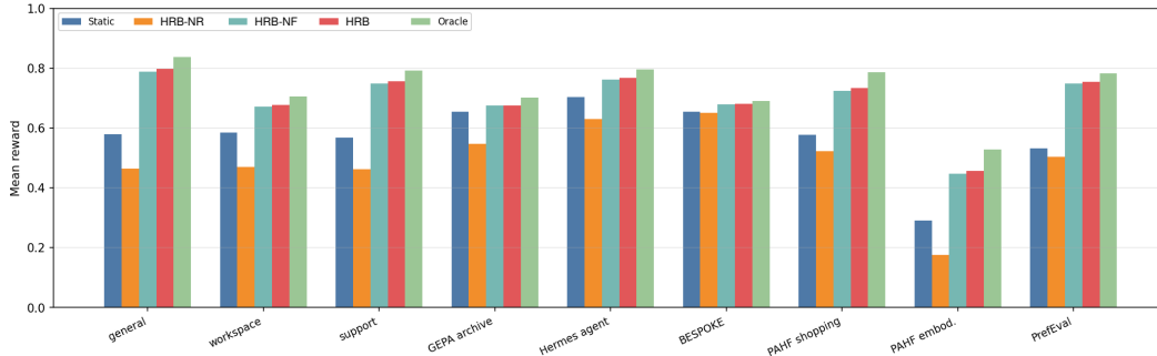
Figure 1: Component ablations of HyperRidge-Base (HRB). Mean reward on nine benchmarks. Within each benchmark, the bars are ordered Static, HRB-NR, HRB-NF, HRB, and Oracle from left to right. HRB-NR and HRB-NF remove routing and reflection from HRB, respectively. HRB uses ordinary ridge, not a learned covariance. The bars show means without uncertainty intervals.
