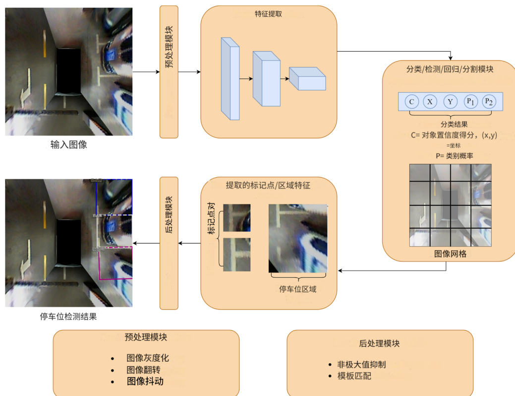
图 2.2 停车位检测的一般流程 [33] Fig 2.2 General Flow for Parking Slot Detection [33]
