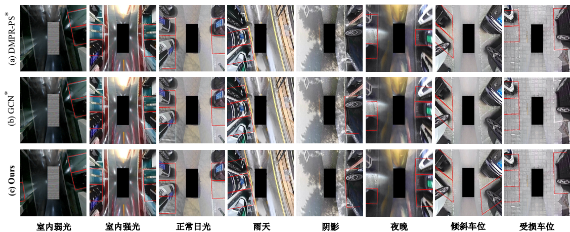
图 3-9 不同复杂场景下的可视化检测结果 Figure 3-9 Qualitative visualization results across various challenging scenes
