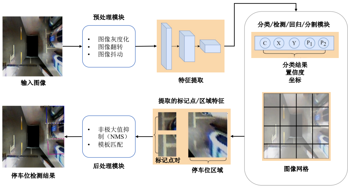
图 2-1 停车位检测的典型流程 [32] Fig 2-1 General flow of parking slot detection [32]
