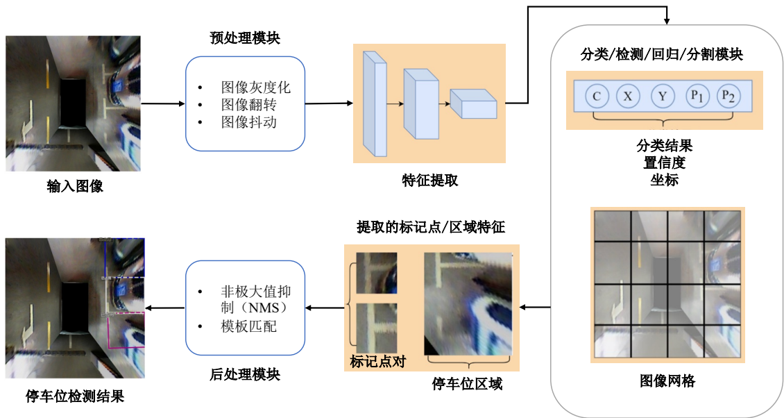
图 2-1 停车位检测的典型流程 [42] Figure 2-1 General flow of parking slot detection [42]
