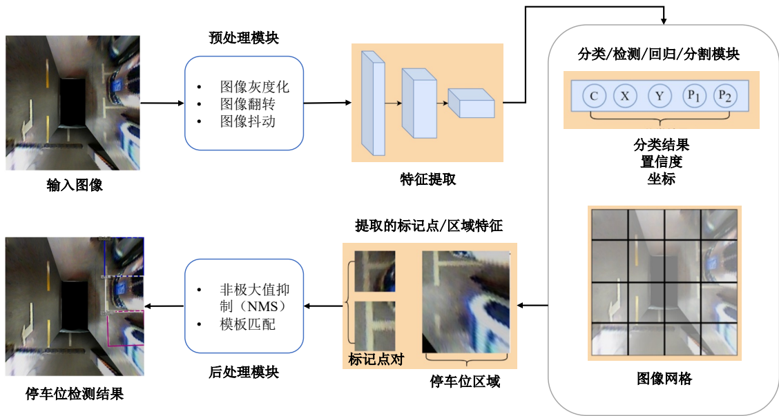
图 2-1 停车位检测的典型流程 [43] Figure 2-1 General flow of parking slot detection [43]
