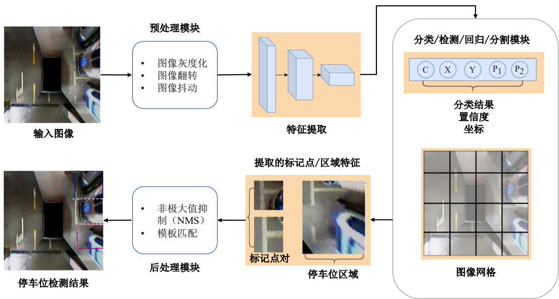
图 2-1 停车位检测的典型流程 [43] Figure 2-1 General flow of parking slot detection [43]
