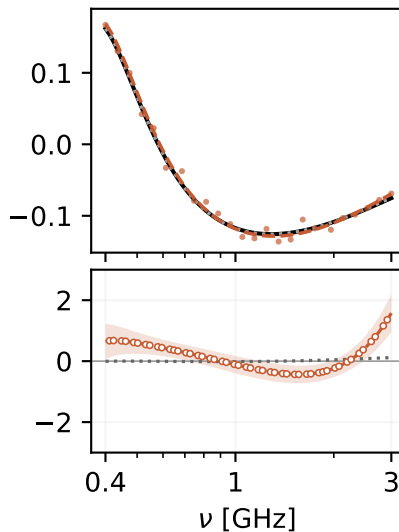
(b) Stokes Q
