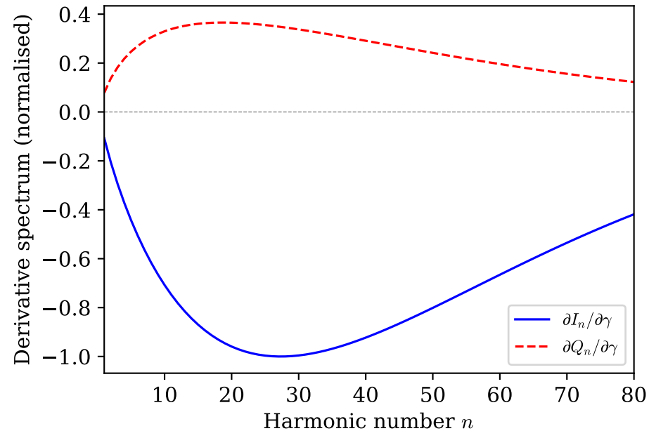
(c) Energy derivative, fixed B ( \gamma_0 = 10.0 )
