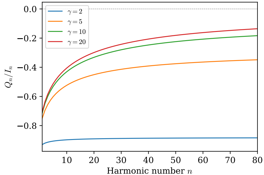
(b) Linear polarisation fraction
