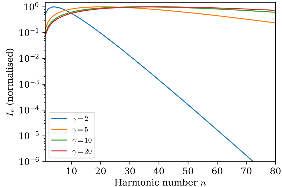
(a) Intensity spectrum I_n
