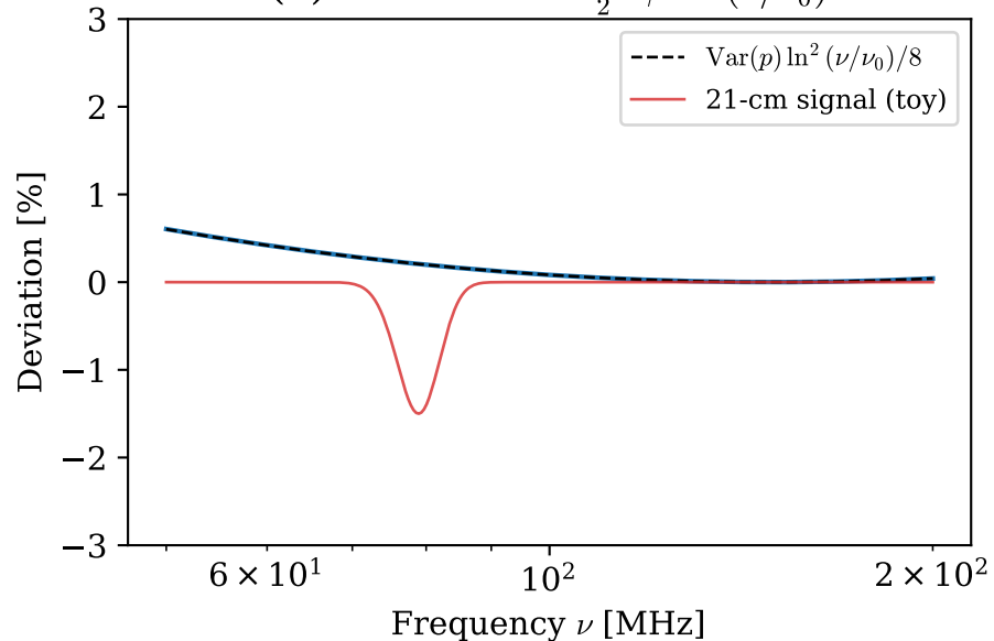
(b) Curvature = \frac{1}{2}\Delta\beta\ln^2(\nu/\nu_0)
