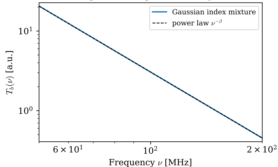
(a) Foreground brightness temperature
