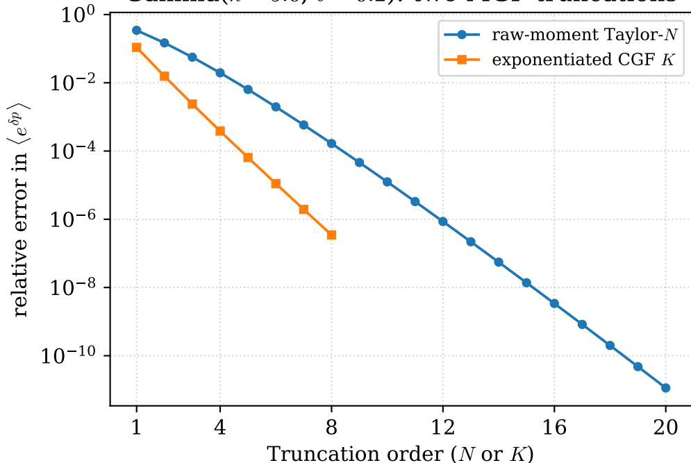
Gamma( k = 5.0 , \theta = 0.2 ): two MGF truncations
