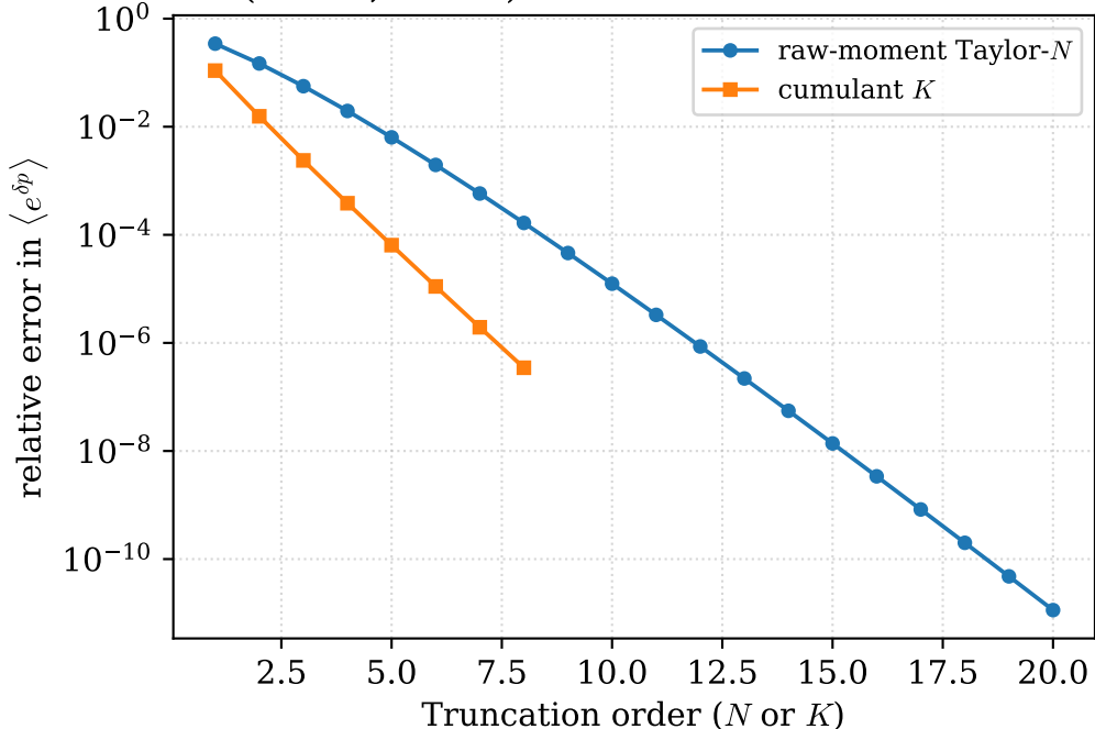
Gamma( k=5.0 , \theta=0.2 ): moment vs cumulant truncation
