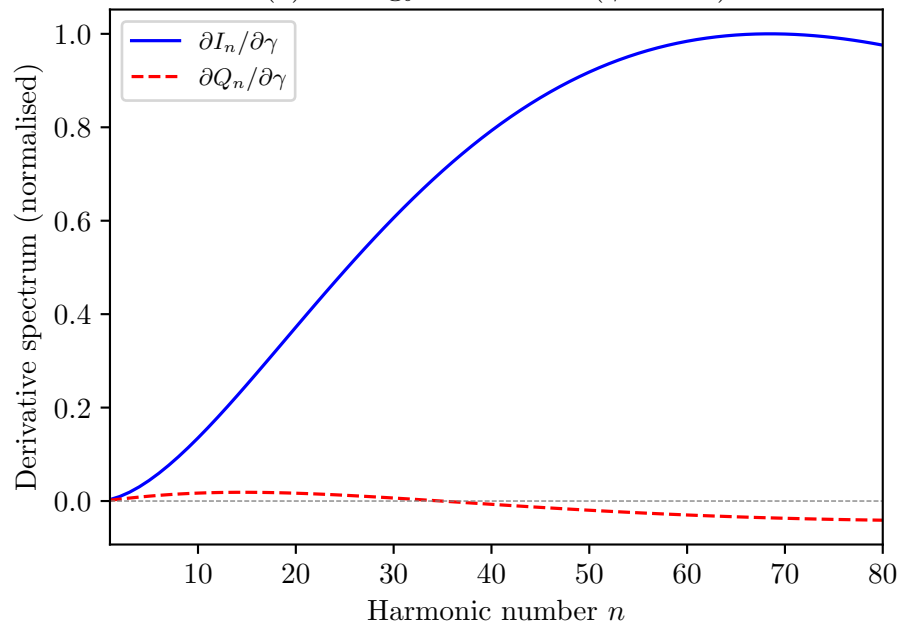
(c) Energy derivative ( \gamma_0 = 10 )
