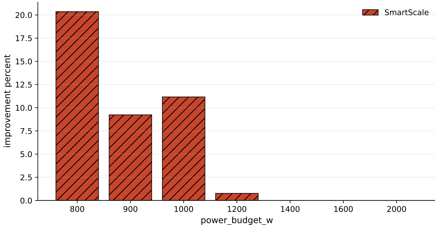
SPEC/tealeaf: improve_vs_max_gpu_pct
