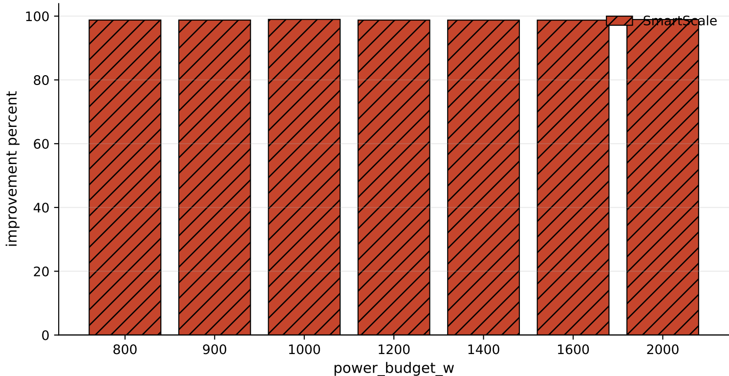
SPEC/hpgmg: improve_vs_max_gpu_pct
