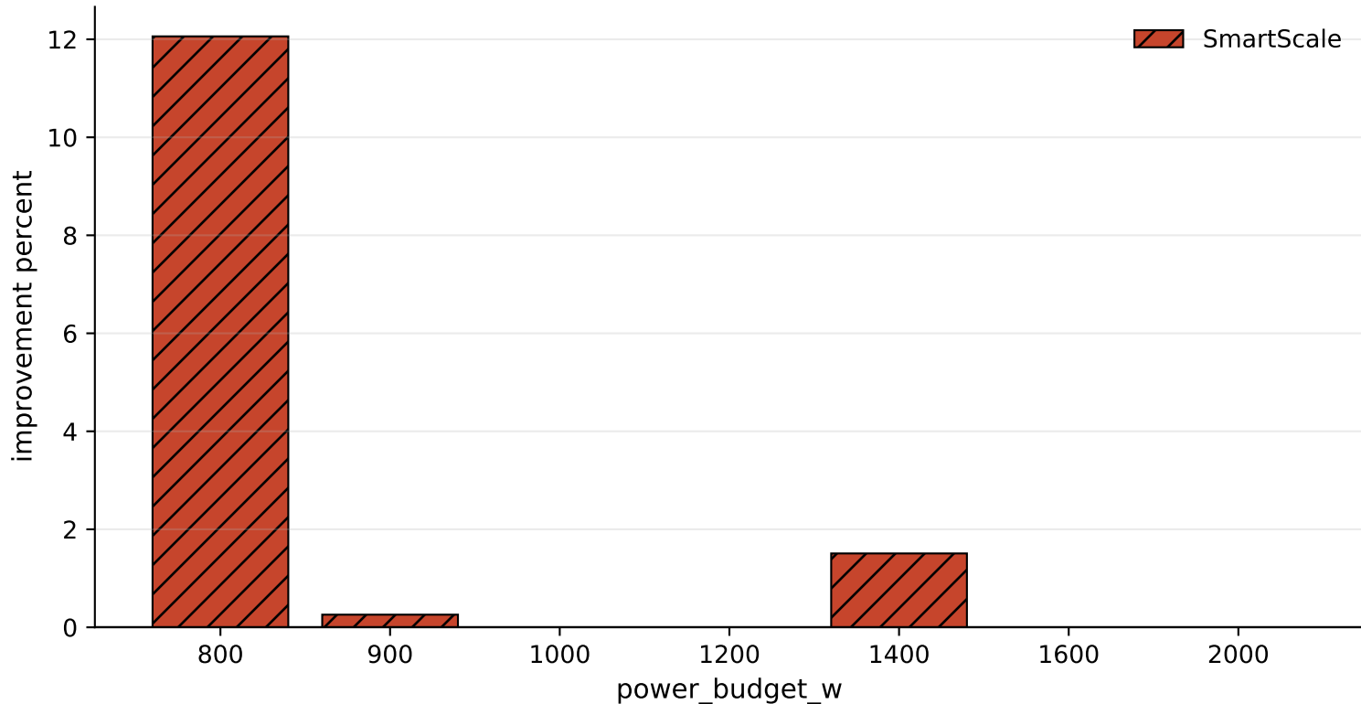
SPEC/cloverleaf: improve_vs_max_gpu_pct
