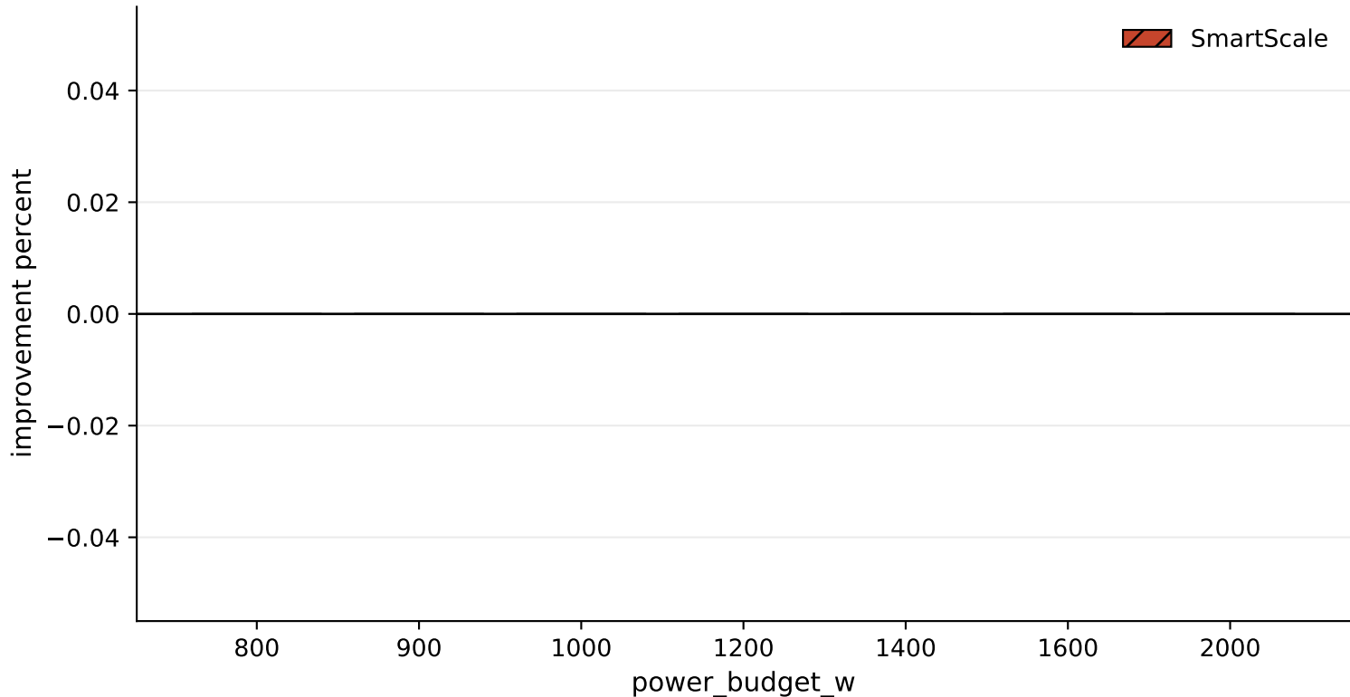
SPEC/minisweep: improve_vs_max_gpu_pct
