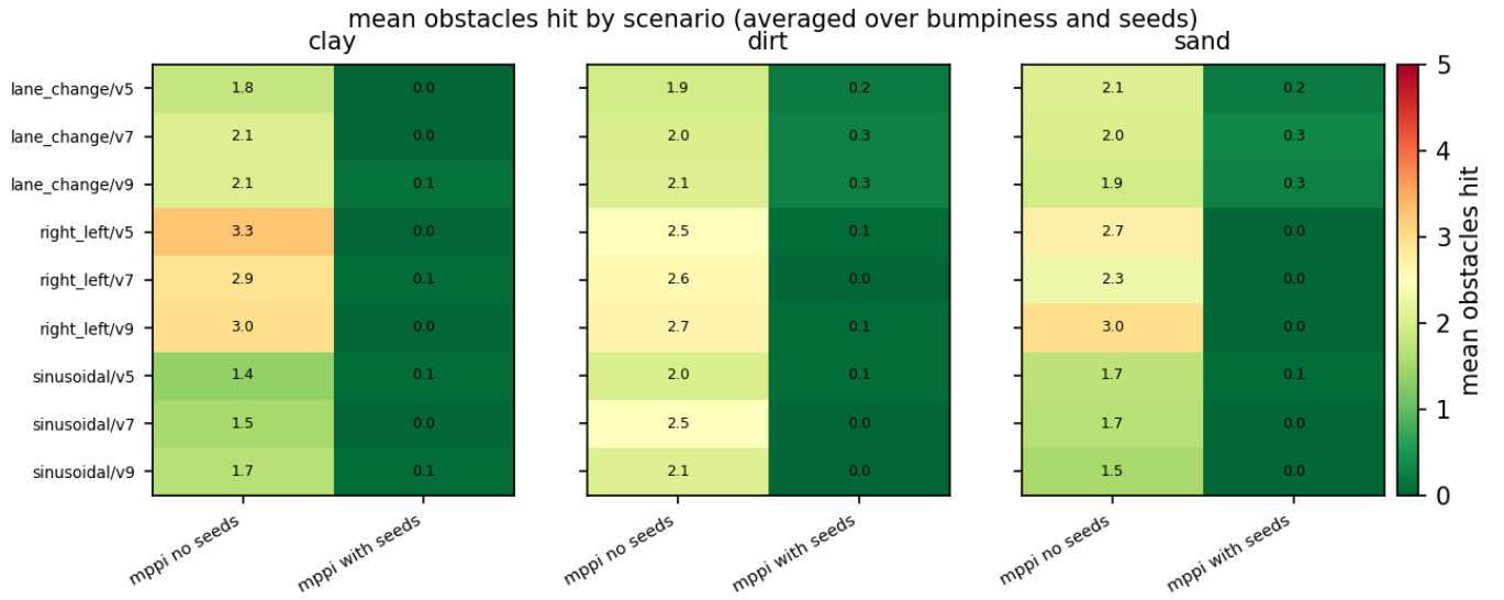
Fig. 20: MPPI seed-trajectory ablation. Removing the seeds eliminates the safety filter’s commitment to evasive maneuvers; the weighted mean then averages over many comparably high-error samples rather than concentrating on a recoverable trajectory.
