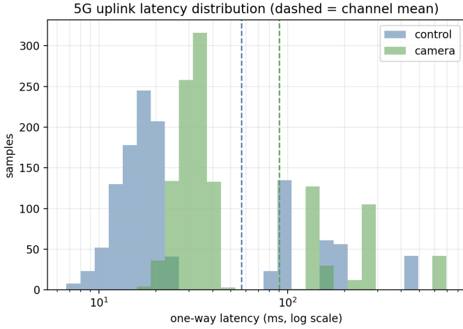
Fig. 22: Learned N-HITS 5G uplink profile applied to the camera and control channels (log- x histogram; dashed lines are channel means). The profile is bimodal: a low-latency good-window bulk (control around 10–25 ms, camera around 30–50 ms), a poor-window cluster near 100–200 ms, and discrete outage spikes at 450 ms (control) and 660 ms (camera). Mean one-way latency is approximately 57 ms (control) and 91 ms (camera).
