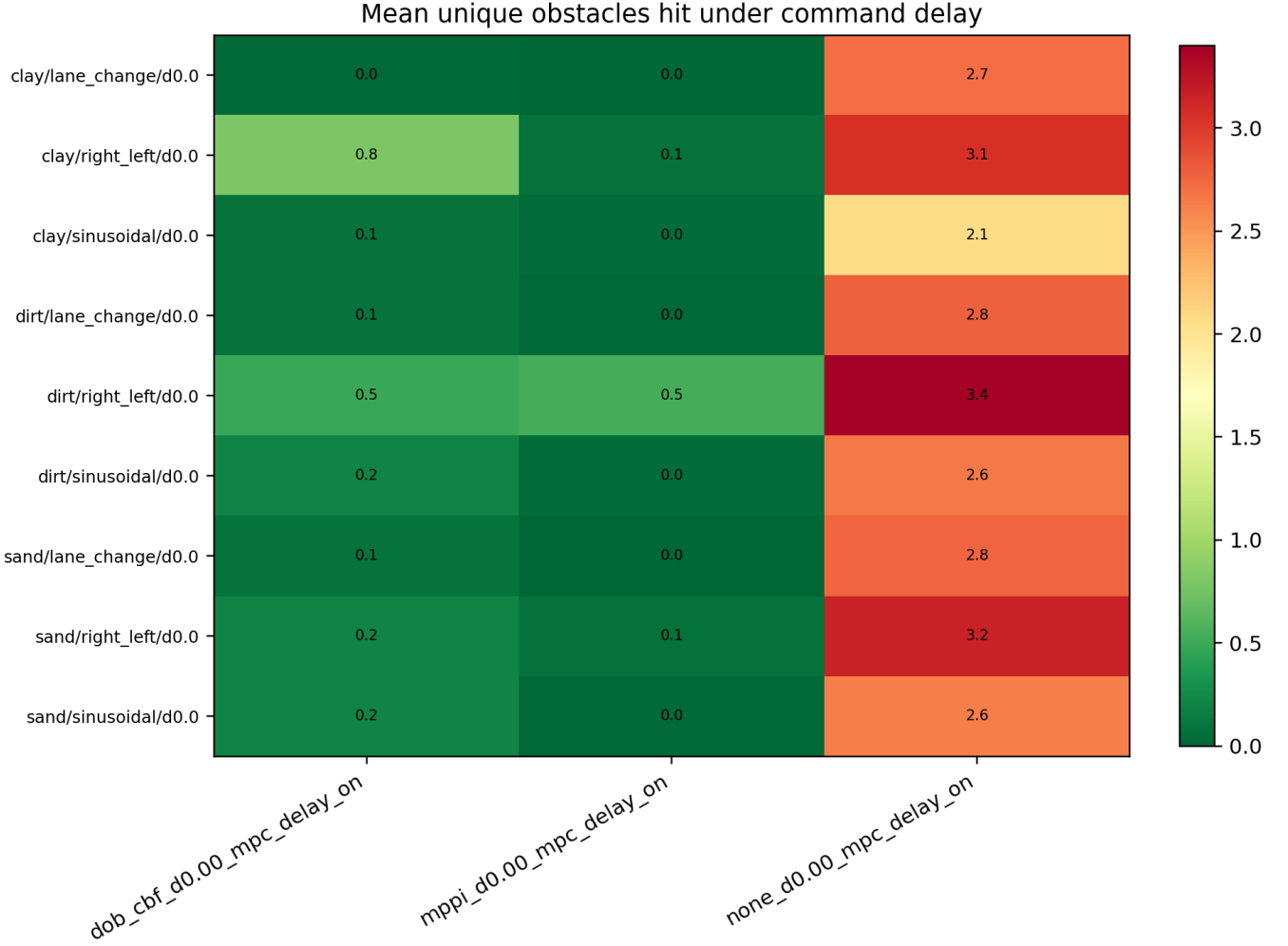
Fig. 23: 5G-profile latency compensation sweep: per-scenario collisions. Aggregate KPIs are in Table XIX.
