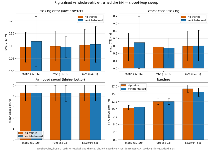
Fig. 4: Aggregate metrics over the 432-run controlled sweep, six surrogates paired by architecture and signature. RMS CTE, worst-case |\text{CTE}| , achieved speed, and solver wall time on the same matrix. Bars are mean \pm s.d. across 72 cells per surrogate. The pre-retrain rig-trained advantage narrows to a static-only effect once architecture is matched and the whole-vehicle training data is LHS-sampled over the same Bekker-Mohr box the rig uses.
