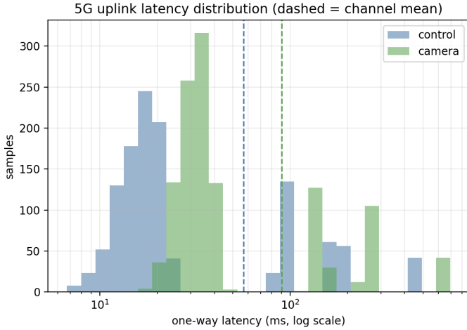
Fig. 22: Learned N-HiTS 5G uplink profile applied to the camera and control channels (log- x histogram; dashed lines are channel means). The profile is bimodal: a low-latency bulk (control around 10–25 ms, camera around 30–50 ms), a higher-latency cluster near 100–200 ms, and discrete outage spikes at 450 ms (control) and 660 ms (camera). Mean one-way latency is approximately 57 ms (control) and 91 ms (camera).
