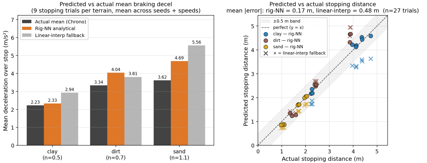
Fig. 24: Validation of the warning system’s analytical brake-deceleration table against actual Chrono SCM stopping behaviour (27 trials, 3 terrains \times 3 initial speeds \times 3 seeds). Left: mean deceleration over each stop. The rig-NN analytical estimate (orange) matches the Chrono mean (black) closely on clay and slightly over-predicts on dirt and sand; the original linear-interp fallback (grey) under-predicts on clay and over-predicts on sand. Right: predicted vs actual stopping distance with the \pm 0.5 m band shaded. Rig-NN points (circles) cluster tighter to y = x than linear-interp ( \times , scatter); mean |\Delta d_{\text{stop}}| is 0.17 m analytical vs 0.45 m linear-interp.
