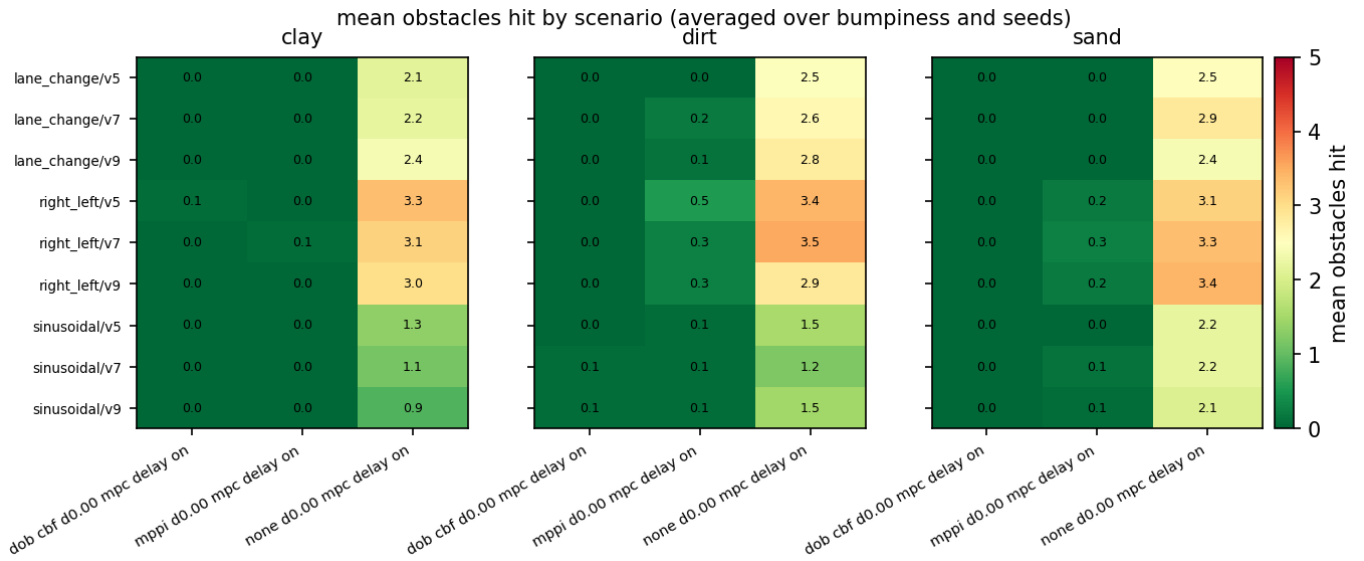
Fig. 22: 5G-profile latency compensation sweep: per-scenario collisions. Aggregate KPIs are in Table XVII.
