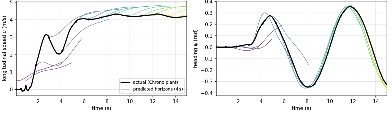
Fig. 6: Open-loop NMPC prediction versus the Chrono plant for a representative firm-sand sinusoidal run (deployed vehicle-rate surrogate). Each 4 s predicted horizon (thin, colour-graded by launch time; dots mark the launch point) branches off the actual plant trace (bold black). Left: longitudinal speed u — the horizons run above the plant and the gap widens along the horizon, the F_x motion-resistance bias the throttle disturbance observer absorbs online. Right: heading \psi — the horizons hug the plant, so the path geometry (lateral F_y ) is predicted accurately. Aggregate drifts across the 18-run matrix are quoted in the text ( \leq 0.15 rad heading over 4 s versus a speed bias growing to \approx 1 m/s on firm sand).
