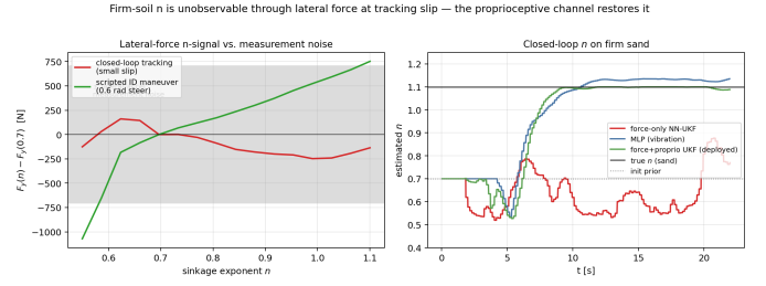
Fig. 9: Force observability of the sinkage exponent n . Left : the lateral-force n -signal |F_y(n=1.1) - F_y(n=0.7)| against the lateral-accel measurement-noise band ( m R_{a_y} \approx 770\text{ N} , R_{a_y} = 0.3\text{ m/s}^2 ). At closed-loop small-slip path tracking the signal ( \approx 132\text{ N} ) stays inside the band — n is unobservable from force — whereas a scripted 0.6 rad maneuver escapes it ( \approx 743\text{ N} , with dF_y/dn \approx 16\times larger). Right : closed-loop \hat{n}(t) on firm sand: the force-only NN-UKF, lacking an observable force signal, drifts in the wrong direction, while the deployed Fused-UKF tracks the true n by leaning on its proprioceptive channel.
