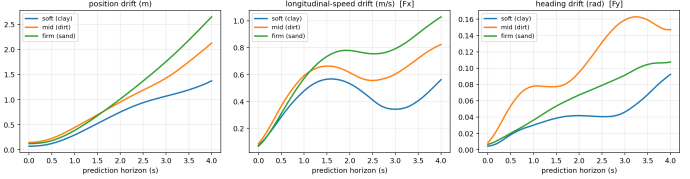
Fig. 6: Open-loop NMPC prediction drift versus the Chrono plant, by horizon time and terrain (mean over 18 runs, deployed vehicle-rate surrogate). Left: front-axle position drift. Middle: longitudinal-speed drift — the deployment measure of F_x prediction quality. Right: heading drift (lateral, F_y ). The model predicts heading well ( \leq 0.15 rad over 4 s) but carries a persistent \approx 0.5 m/s speed bias, so F_x is the dominant prediction error.
