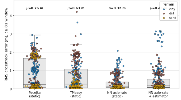
Fig. 3: Same benchmark, RMS CTE distribution per variant. Box plots show interquartile range and median across all 405 runs per variant; jittered scatter points are coloured by terrain (clay, dirt, sand). The two analytical baselines (Pacejka, TMeasy) carry long right tails driven by a few dirt cases at higher v_{\text{ref}} ; both neural variants compress the distribution sharply. The estimator-on variant nearly matches the matched-prior static row, the deployable claim of Sec. III-C.
