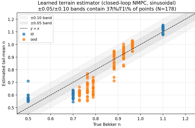
Fig. 7: Learned (sliding-window MLP) terrain estimator: true vs. estimated Bekker n (tail-window mean) on the closed-loop sinusoidal benchmark, evaluated within the estimator's training envelope (bumpiness \in \{0, 4\} ). Blue = in-distribution canonical soils (clay/dirt/sand); orange = Bekker-jittered out-of-distribution soils ( n sampled in [0.40, 1.30] , other five Bekker parameters perturbed \pm 30\text{--}50\% ). The \pm 0.05 / \pm 0.10 bands around y = x contain 40% / 68% of points. The estimator tracks the diagonal across the deployment range, with a mild systematic over-prediction in the lowest- n (clay) bin (mean estimate 0.59 vs. true 0.50). See the out-of-envelope note in the text for behaviour at bumpiness 8.
