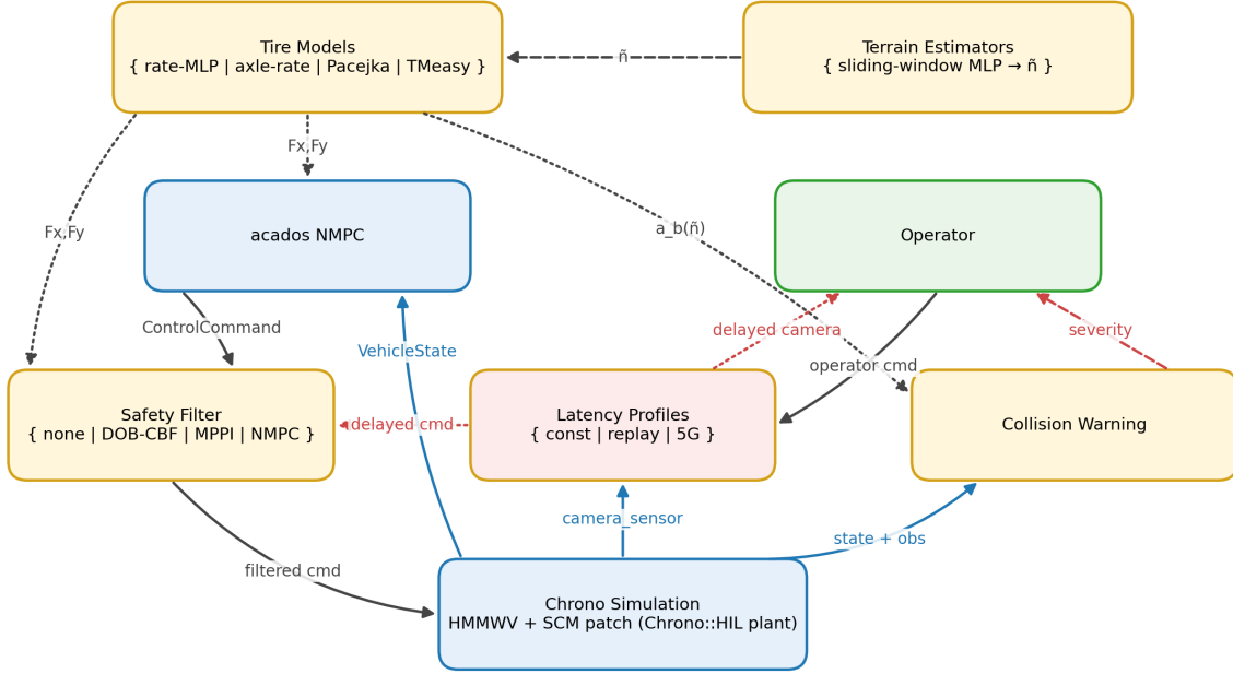
Fig. 1: Shared-control framework. Yellow nodes are in-process swap points resolved by the corresponding registry; blue/green nodes are process-boundary or operator endpoints. Solid arrows are runtime data flow over ZeroMQ; dashed arrows are the latency-affected operator paths; dotted arrows are tire-surrogate queries (build-time CasADi export plus per-tick safety-filter rollouts).
