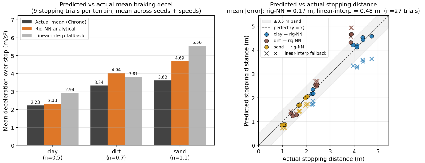
Fig. 22: Validation of the warning system's analytical brake-deceleration table against actual Chrono SCM stopping behaviour (27 trials, 3 terrains \times 3 initial speeds \times 3 seeds). Left: mean deceleration over each stop. The rig-NN analytical estimate (orange) matches the Chrono mean (black) closely on clay and slightly over-predicts on dirt and sand; the original linear-interp fallback (grey) under-predicts on clay and over-predicts on sand. Right: predicted vs actual stopping distance with the \pm 0.5 m band shaded. Rig-NN points (circles) cluster tighter to y = x than linear-interp ( \times , scatter); mean |\Delta d_{\text{stop}}| is 0.17 m analytical vs 0.45 m linear-interp.
