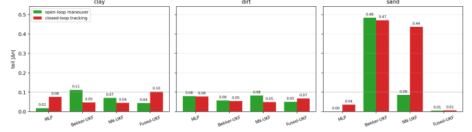
Fig. 7: Open-loop excitation vs. closed-loop tracking, all four estimators, canonical soils (tail |\Delta n| ). A scripted 0.6 rad sine-steer maneuver (green) is compared to closed-loop NMPC path-tracking (red). On firm sand the force-only NN-UKF goes 0.44 \rightarrow 0.09 — observability -limited, a dedicated maneuver resolves it — whereas the Bekker-UKF remains \approx 0.47 in both ( model -limited: its analytical contact law is inaccurate on sand). The proprioceptive MLP is excitation-agnostic (0.04 \rightarrow 0.00), and the deployed Fused-UKF is accurate in both ( \approx 0.01 ), so it needs no dedicated maneuver at runtime (cf. Sec. IV-B).
