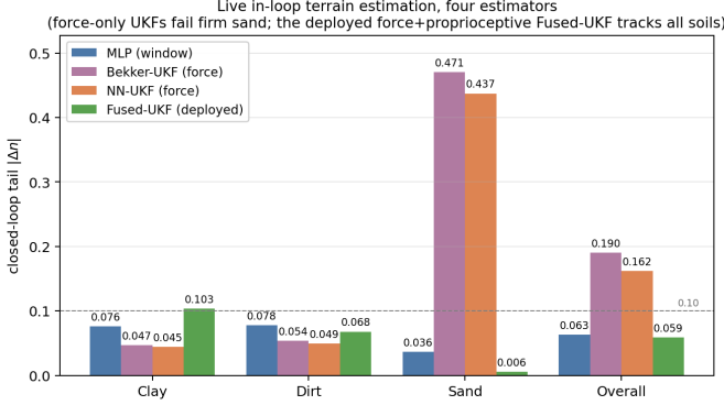
Fig. 10: Deployment summary: tail |\Delta n| over the canonical clay/dirt/sand presets and the overall mean for the proprioceptive MLP, the analytical Bekker-UKF, the force-only NN-UKF, and the deployed Fused-UKF (all run live in the closed loop, v \in \{5, 7\} m/s, three seeds). The force-only UKFs fail firm sand; the covariance-fused proprioceptive channel makes n observable, so the Fused-UKF is best overall (0.059) with no hand-tuned gate.
