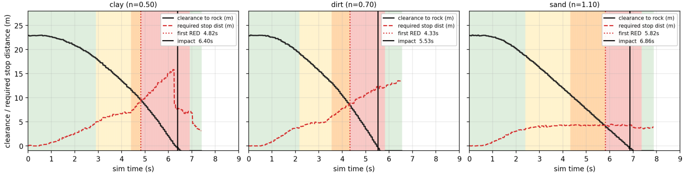
Fig. 23: Severity escalation over time for one representative blind-drive run per terrain at 150 ms one-way delay. Background shading is the live severity band (GREEN → YELLOW → ORANGE → RED); curves are the chassis clearance to the rock (solid) and the warning system’s running stopping-distance estimate (dashed). The first RED fires when the clearance curve drops to the stopping-distance curve.
