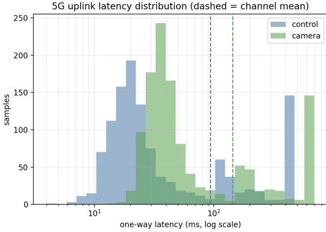
Fig. 20: Learned N-HiTS 5G uplink profile applied to the camera and control channels (log- x histogram; dashed lines are channel means). The profile is bimodal: a low-latency good-window bulk (control around 10–25 ms, camera around 30–50 ms), a poor-window cluster near 100–200 ms, and discrete outage spikes at 450 ms (control) and 660 ms (camera). Mean one-way latency is approximately 94 ms (control) and 144 ms (camera).
