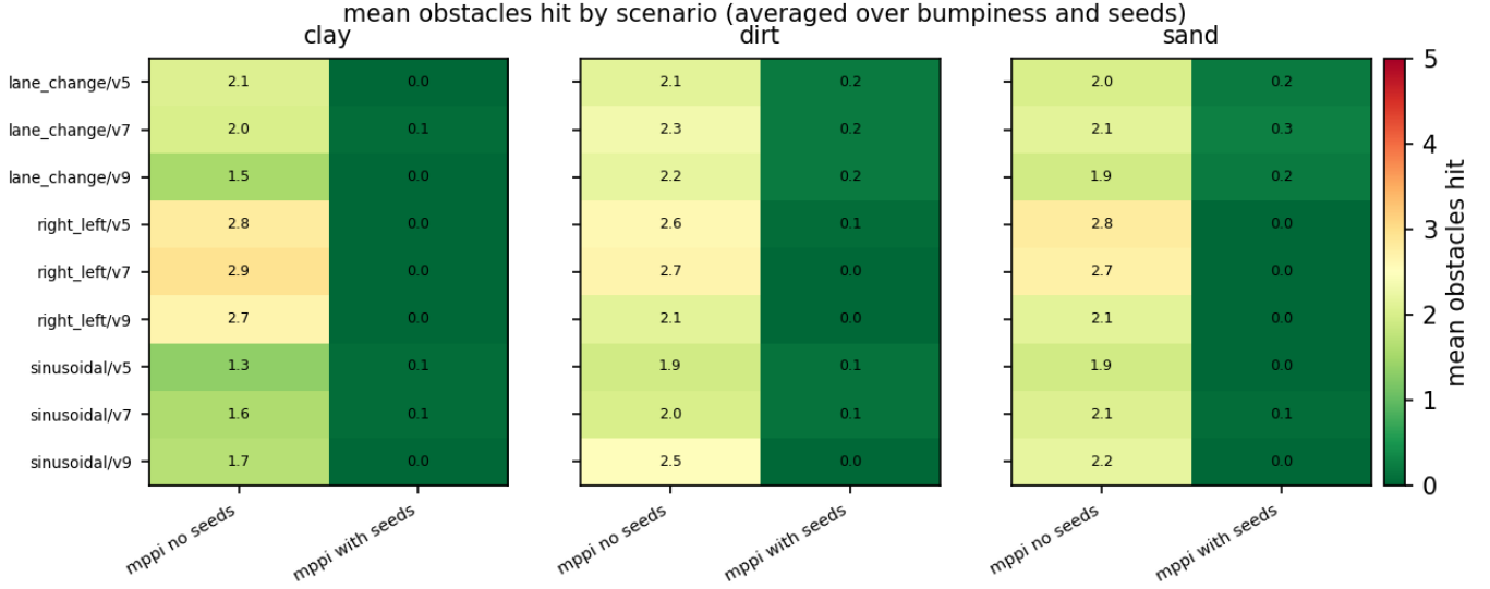
Fig. 18: MPPI seed-trajectory ablation. Removing the seeds eliminates the safety filter’s commitment to evasive maneuvers; the weighted mean then averages over many comparably high-error samples rather than concentrating on a recoverable trajectory.
