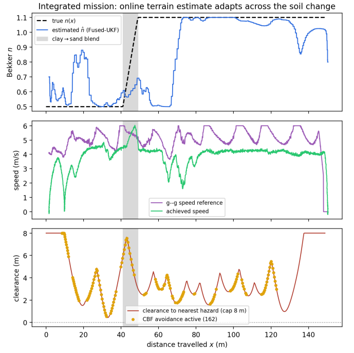
Fig. 27: Integrated mission: the whole stack on one run, under the learned 5G latency, across a clay \rightarrow sand soil change (grey band) through a rock field. Top: the online terrain estimate \hat{n} (blue) tracks the true n(x) (dashed) across the soil boundary. Middle: achieved speed (green) tracks the terrain-aware g-g reference (purple). Bottom: clearance to the nearest hazard (capped at 8 m) dips at each rock, with the DOB-CBF binding-constraint avoidance steps marked; zero collisions over the traverse.
