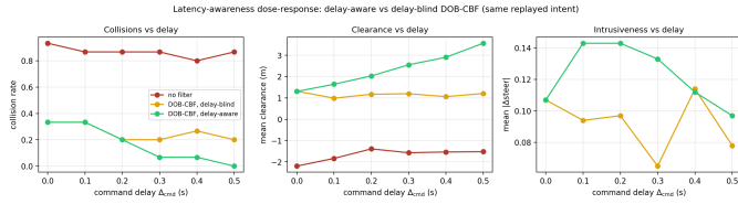
Fig. 23: Latency-awareness dose-response. The same adversarial intents are replayed with the command path delayed by \Delta_{\text{cmd}} , the DOB-CBF filter either told that delay (aware) or not (blind), swept over six delays. At zero delay the two coincide (nothing to be aware of); the gap grows with delay — by 0.5 s awareness removes the residual collisions the delay-blind filter still suffers, at comparable intrusiveness. 90 deterministic cells per variant.
