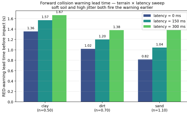
Fig. 25: Forward collision warning lead time before impact in the blind-drive sweep (no MPC, no safety filter, fixed throttle into a single rock). Both the terrain-conditioned brake budget and the latency-conditioned operator-reaction budget enlarge the required stopping distance and therefore advance the first RED warning: soft soil (clay) gets the longest lead, and within every terrain the lead grows monotonically with the configured one-way delay.
