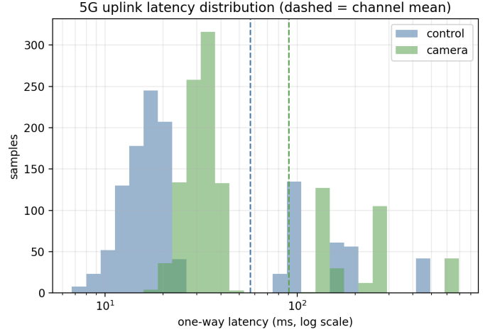
Fig. 20: Learned N-HiTS 5G uplink profile applied to the camera and control channels (log- x histogram; dashed lines are channel means). The profile is bimodal: a low-latency bulk (control around 10–25 ms, camera around 30–50 ms), a higher-latency cluster near 100–200 ms, and discrete outage spikes at 450 ms (control) and 660 ms (camera). Mean one-way latency is approximately 57 ms (control) and 91 ms (camera).
