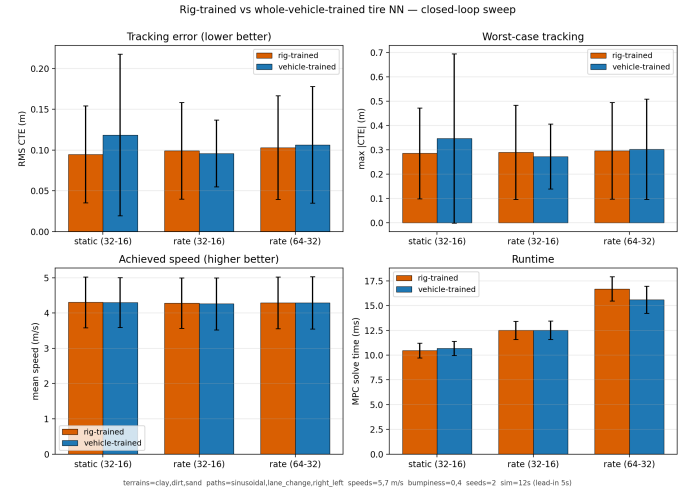
Fig. 4: Aggregate metrics over the 432-run controlled sweep, six surrogates paired by architecture and signature. RMS CTE, worst-case |CTE|, achieved speed, and solver wall time on the same matrix. Bars are mean \pm s.d. across 72 cells per surrogate. The pre-retrain rig-trained advantage narrows to a static-only effect once architecture is matched and the whole-vehicle training data is LHS-sampled over the same Bekker-Mohr box the rig uses.
