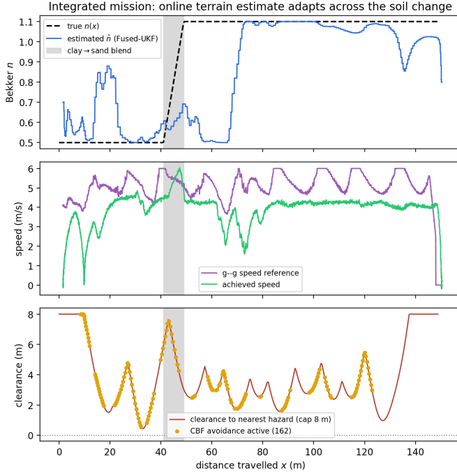
Fig. 26: Integrated mission: the whole stack on one run, under the learned 5G latency, across a clay \rightarrow sand soil change (grey band) through a rock field. Top: the online terrain estimate \hat{n} (blue) tracks the true n(x) (dashed) across the soil boundary. Middle: achieved speed (green) tracks the terrain-aware g-g reference (purple). Bottom: clearance to the nearest hazard (capped at 8 m) dips at each rock, with the DOB-CBF binding-constraint avoidance steps marked; zero collisions over the traverse.
