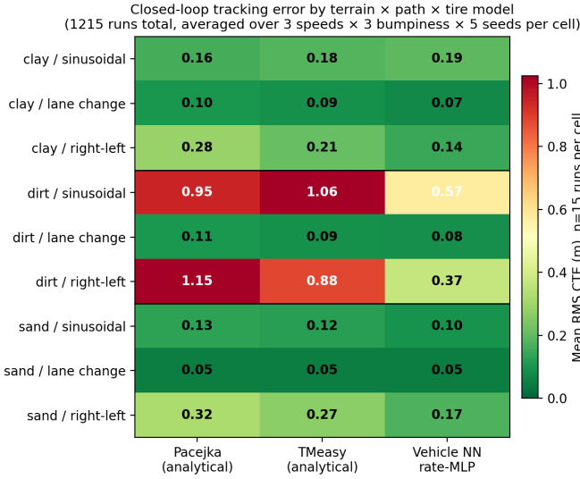
Fig. 2: Closed-loop RMS CTE per (terrain, path) cell across the broader 1215-run sweep (3 speeds × 3 bumpiness × 5 seeds per cell). The analytical baselines (Pacejka, TMeasy) track well on clay and sand but diverge on dirt/sinusoidal ( \sim 1.0 m) and dirt/right-left (0.9–1.2 m), where the curvature-limited reference combines with off-nominal sinkage to produce a regime the analytical force laws do not cover even after SCM calibration. The Vehicle NN rate-MLP suppresses those tails to 0.4–0.6 m while matching the calibrated baselines on the benign cells. This per-scenario view is what motivates the live-estimator benchmark in Sec. III-C.
