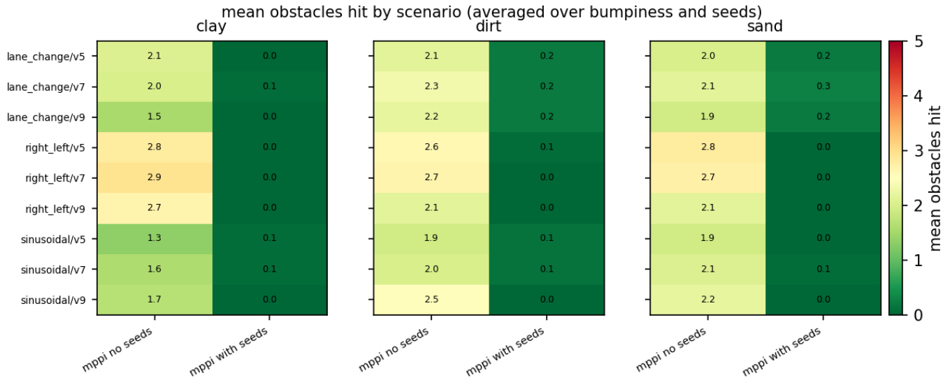
Fig. 19: MPPI seed-trajectory ablation. Removing the seeds eliminates the safety filter’s commitment to evasive maneuvers; the weighted mean then averages over many comparably high-error samples rather than concentrating on a recoverable trajectory.
