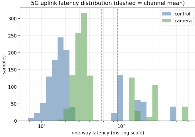
Fig. 20: Learned N-HiTS 5G uplink profile applied to the camera and control channels (log- x histogram; dashed lines are channel means). The profile is bimodal: a low-latency bulk (control around 10–25 ms, camera around 30–50 ms), a higher-latency cluster near 100–200 ms, and discrete outage spikes at 450 ms (control) and 660 ms (camera). Mean one-way latency is approximately 57 ms (control) and 91 ms (camera).
