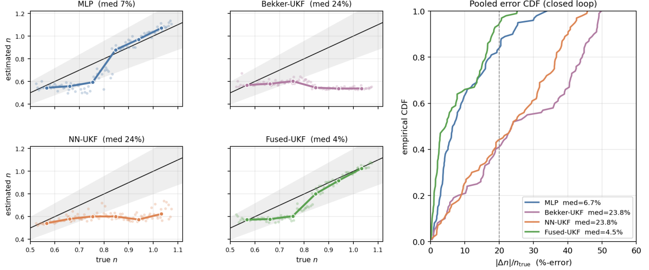
Fig. 12: Closed-loop terrain-estimator benchmark on 100 soils swept along the clay–dirt–sand Bekker–Mohr manifold in Chrono SCM (seed 42, n \in [0.52, 1.08] ); the other five soil parameters follow the preset manifold with \pm 8\% jitter — the parameter-known setting in which the force-dominant exponent n is estimated, and the soil model our estimator reconstructs from \hat{n} ), all run live under closed-loop NMPC sinusoidal path-tracking at 5 m/s. Left, four panels: estimated n versus true n per backend, where faded points are individual soils, the bold line is the binned median, and the black diagonal with its \pm 20\% band is the target. The proprioceptive MLP and the deployed Fused-UKF track the diagonal (fitted slope 1.25 and 1.07), whereas the force-only NN-UKF and Bekker-UKF saturate near n \approx 0.6 on firm soils (slope 0.15 and -0.11 ) — the closed-loop force-observability limit quantified in Sec. IV-B. Right: pooled empirical CDF of the tail-window |\Delta n|/n_{\text{true}} ; the Fused-UKF holds the tightest distribution and the best fraction within \pm 20\% (dashed line).
