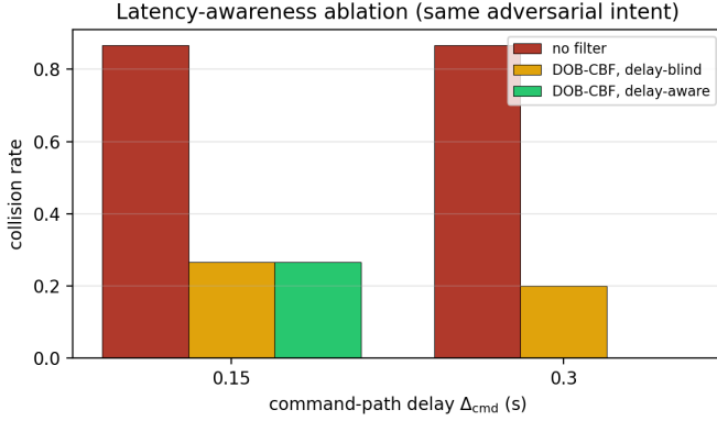
Fig. 22: Latency-awareness ablation. The same adversarial intent is replayed with the command path delayed by \Delta_{\text{cmd}} , the DOB-CBF filter either told that delay (aware) or not (blind). A filter helps at both delays, but knowing the delay matters more as the delay grows: at 0.30 s it removes the residual collisions the delay-blind filter still suffers. 30 deterministic cells per bar.
